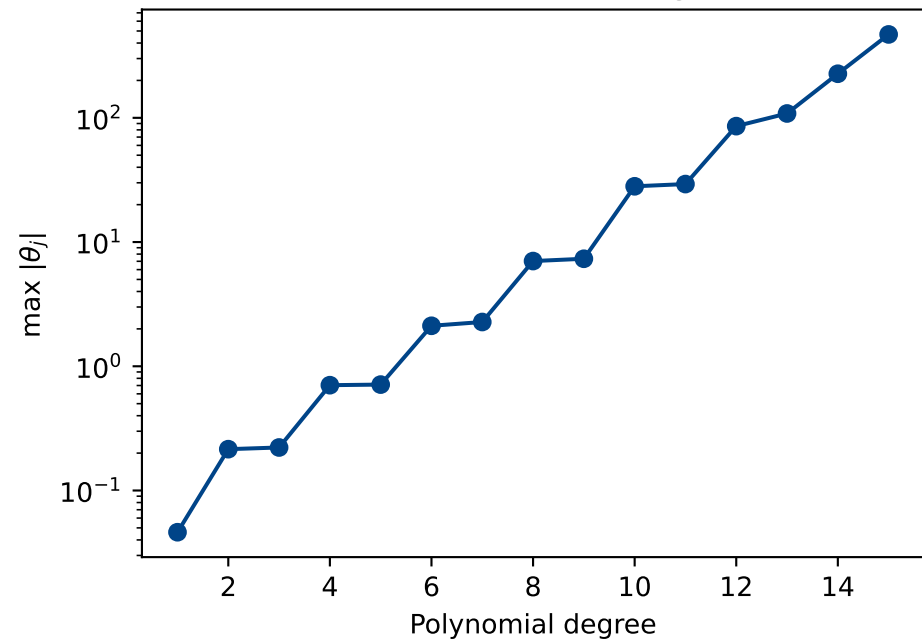
Maximum coefficient magnitude
