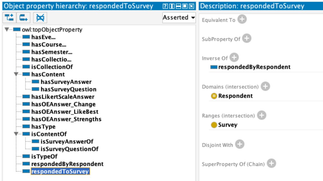
Figure 4.13: Object Property Hierarchies, Domain and Range for Classes
