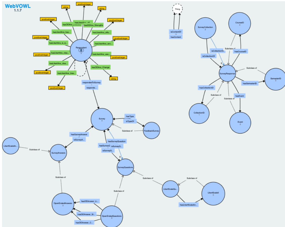
Figure 4.24: WebVOWL for Survey Ontology
