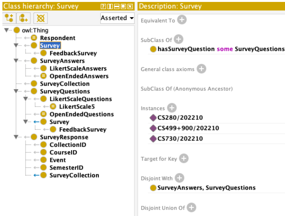
Figure 4.9: Class Hierarchy in Survey Ontology
