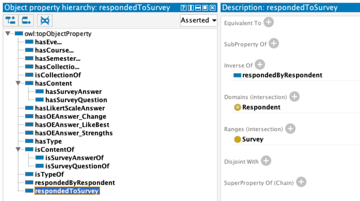
Figure 4.14: Object Property Hierarchies, Domain and Range for Classes
