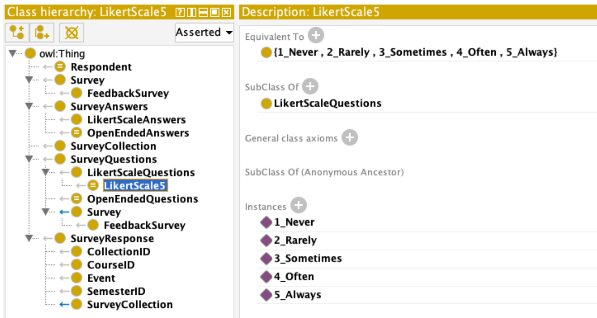
Figure 4.10: “LikertScale5” class in Survey Ontology
