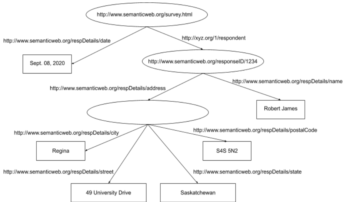
Figure 2.12: RDF Representation in Figure ?? without a URI (blank node) for Address Entity, after RDF Primer [36]
