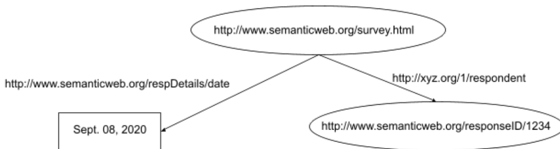
Figura 2.10: RDF Graph for Two Relative Statements, after RDF Primer [36]
