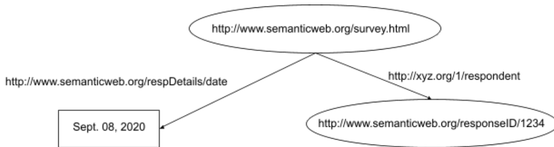
Figure 2.10: RDF Graph for Two Relative Statements, after RDF Primer [34]
