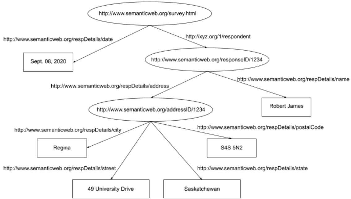
Figure 2.11: Graphical Representation of RDF with Details of the Respondent of the Survey, after RDF Primer [?]
