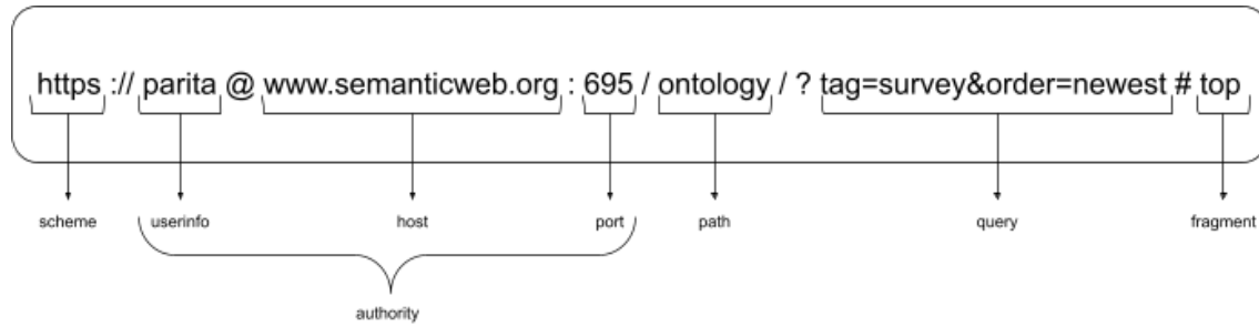
Figure 2.14: Components of an Example of URL, after Berners-Lee et al. [?]
