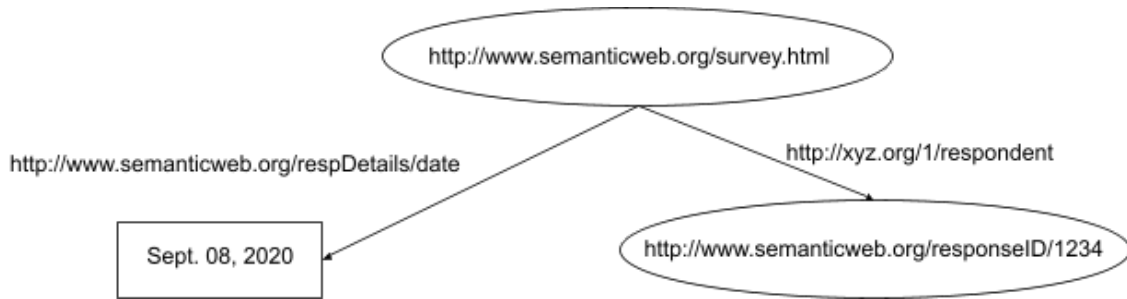
Figure 2.10: RDF Graph for Two Relative Statements, after RDF Primer [?]
