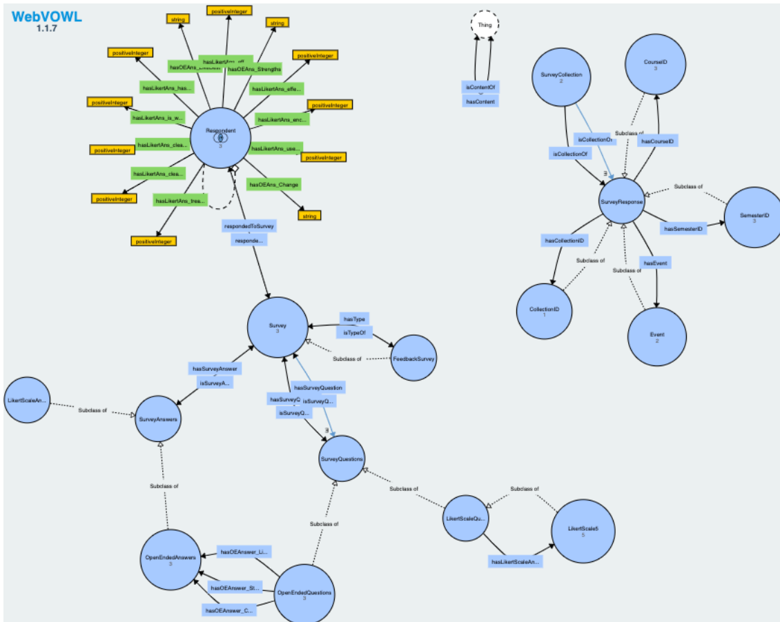
Figure 4.21: WebVOWL for Survey Ontology
