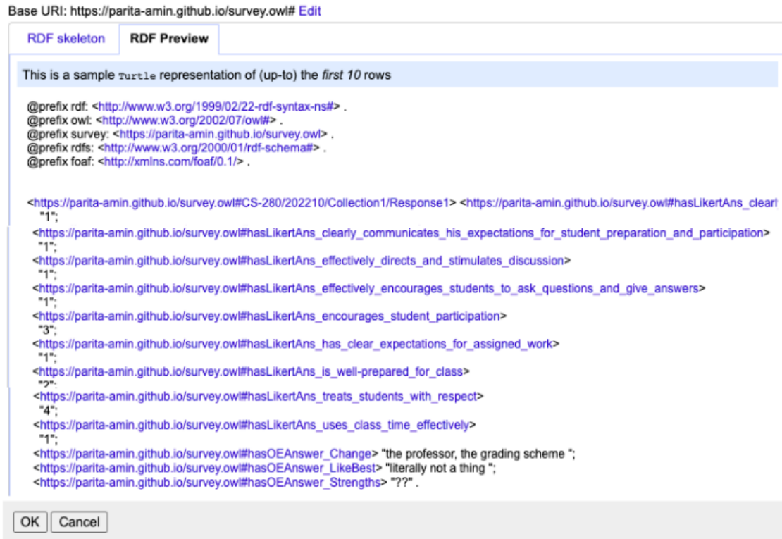
Figure 4.18: RDF Preview for CSV using Survey Ontology
