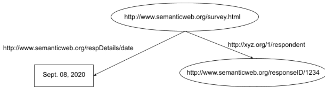
Figure 2.10: RDF Graph for Two Relative Statements, after RDF Primer [35]
