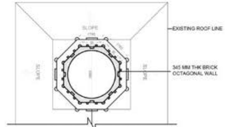
4. PROPOSED PLAN AT UPPER OCTAGONAL BASE
