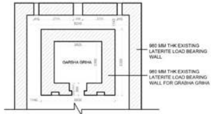
PLAN AT PLINTH LEVEL
