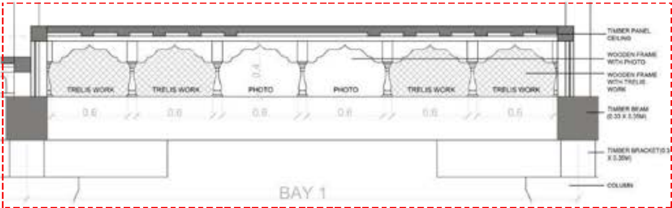
DETAIL AT A : DETAIL FOR BAY 1
