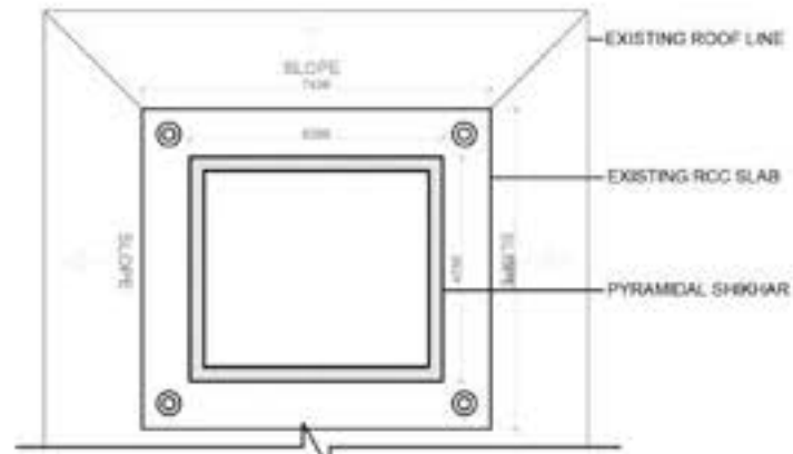
PLAN AT PYRAMIDAL SHIKHAR BASE LEVEL
