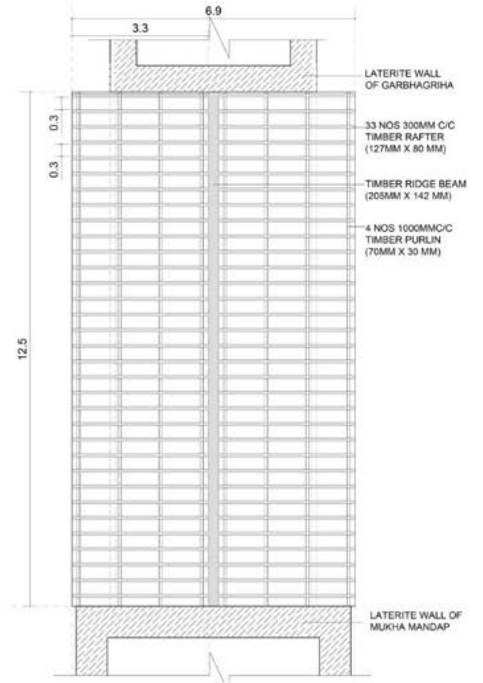
PLAN FOR UPPER ROOF
