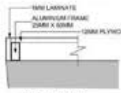
DETAIL AT 'C'
