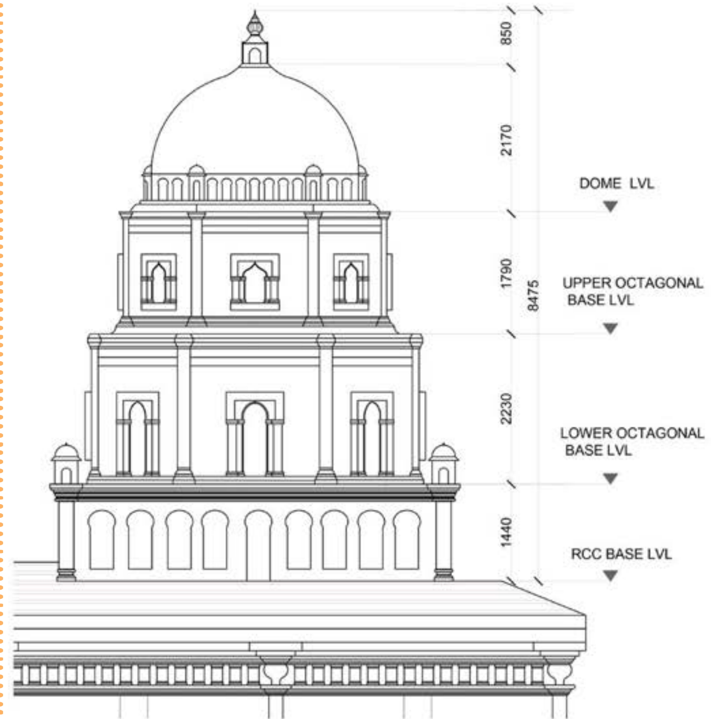
PROPOSED SHIKHAR ELEVATION
