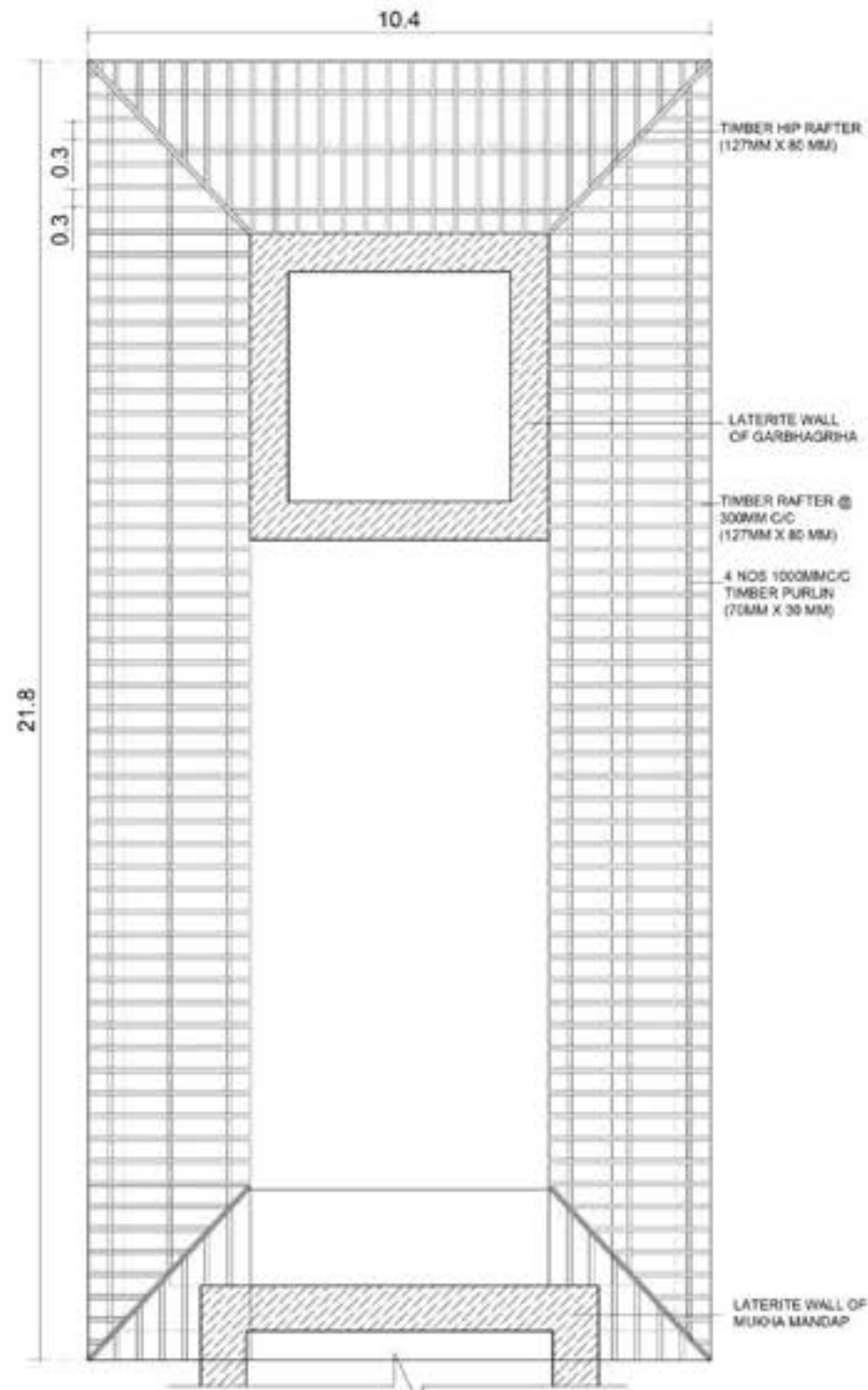
PLAN FOR LOWER ROOF
