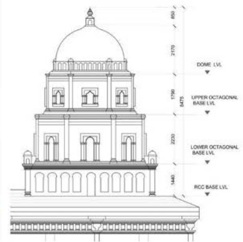
PROPOSED SHIKHAR ELEVATION
