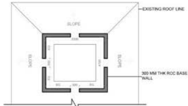
PLAN AT RCC BASE LEVEL
