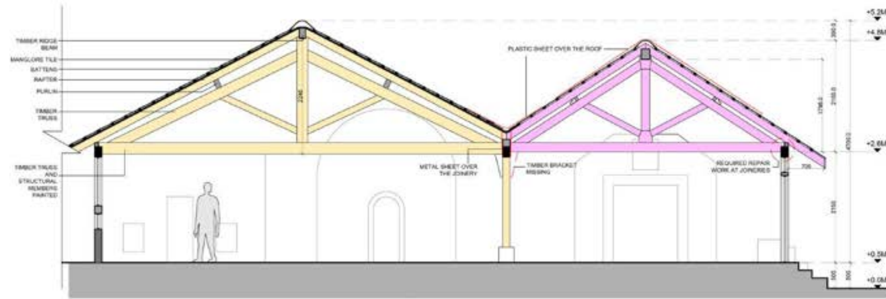
SECTION AA'
