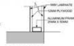
DETAIL AT 'B'
