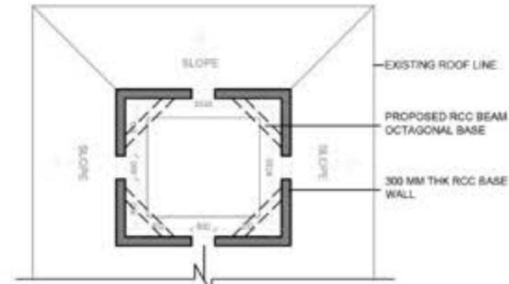
2. PROPOSED PLAN AT RCC BASE LEVEL
