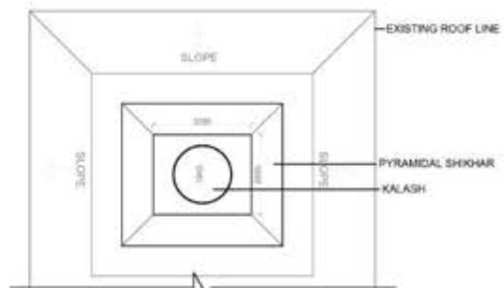
PLAN AT KALASH BASE LEVEL
