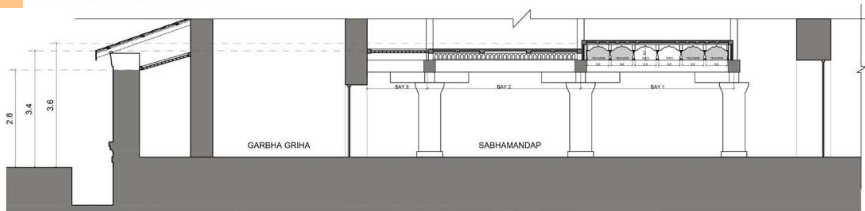
SECTION CC'
