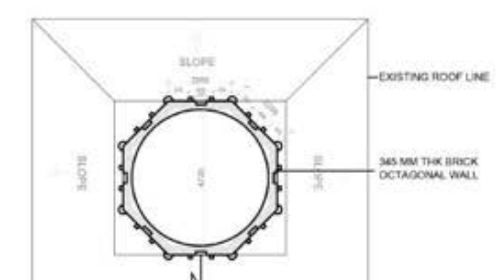
3. PROPOSED PLAN AT LOWER OCTAGONAL BASE
