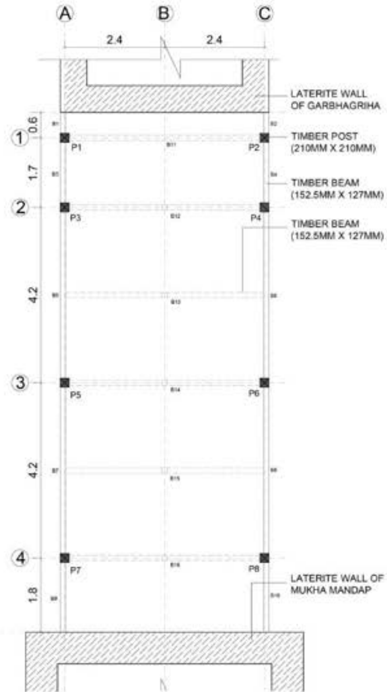
PLAN AT INTERMEDIATE ROOF LEVEL
