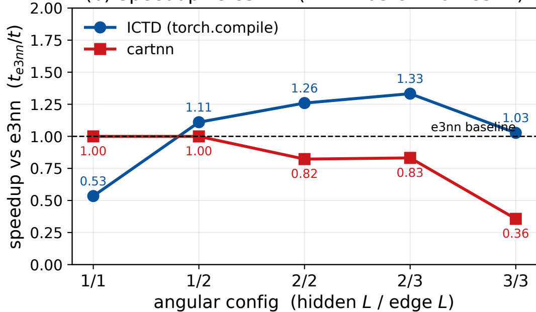
(b) Speedup vs e3nn (>1 = faster than e3nn)
