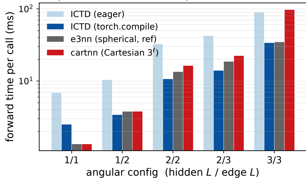
(a) Operator forward time (fp32, C=64, E=100,000)
