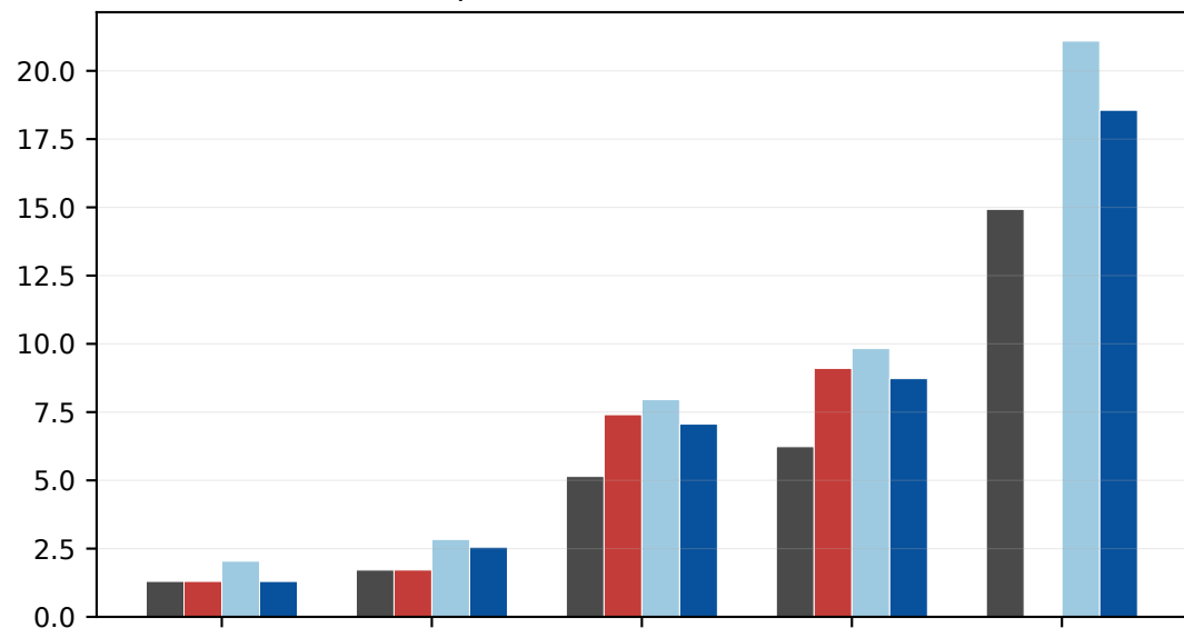
fp64 forward+backward
