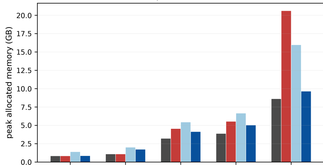
fp64 forward
