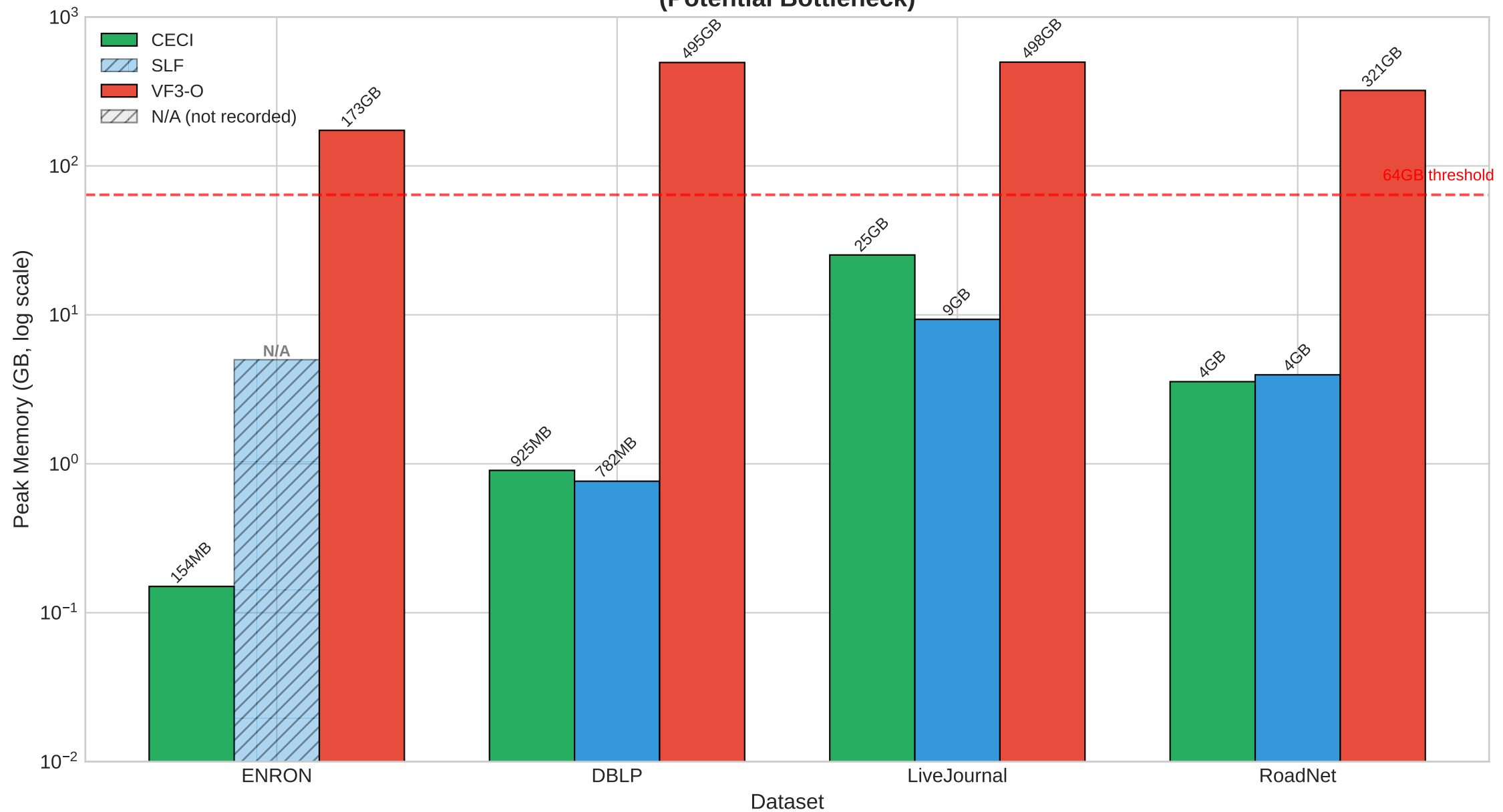
RQ3: Memory Usage - VF3-O Uses 100-500GB (Potential Bottleneck)
