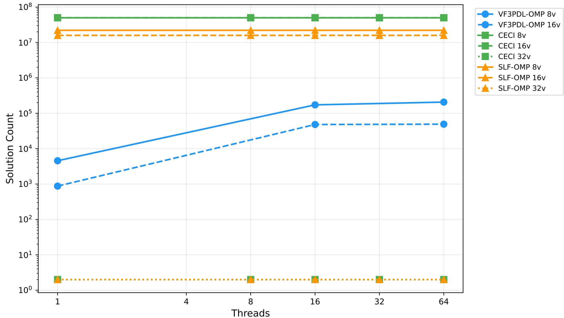
ROADNET - Dense Solution Counts
