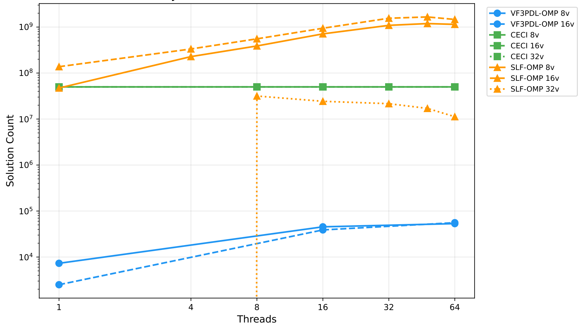
LIVEJOURNAL - Dense Solution Counts
