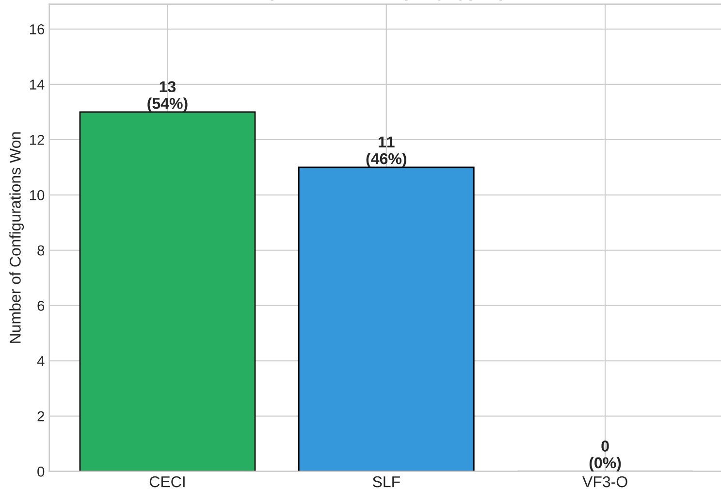
RQ2: Algorithm Wins Across All 24 Configurations (4 datasets × 6 query types)
