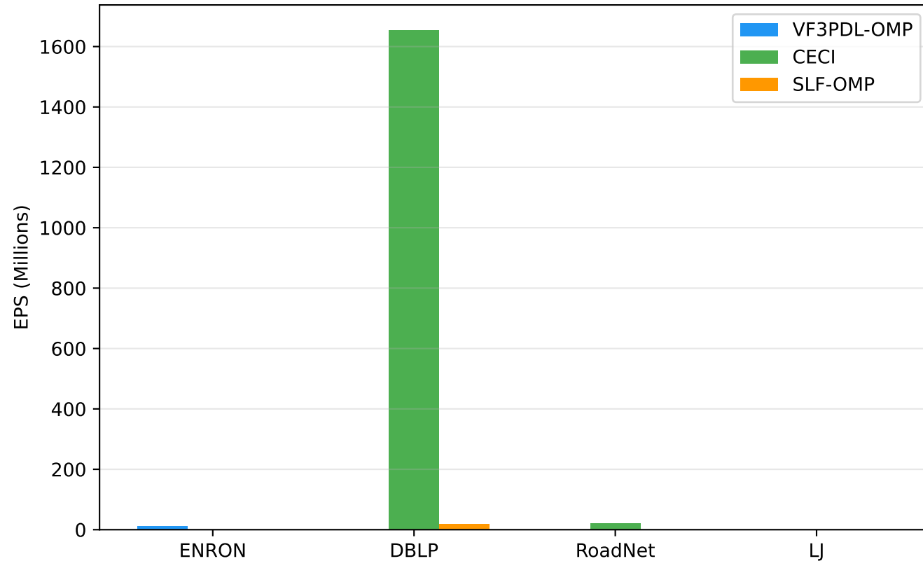
Sparse Queries @ 64 Threads
