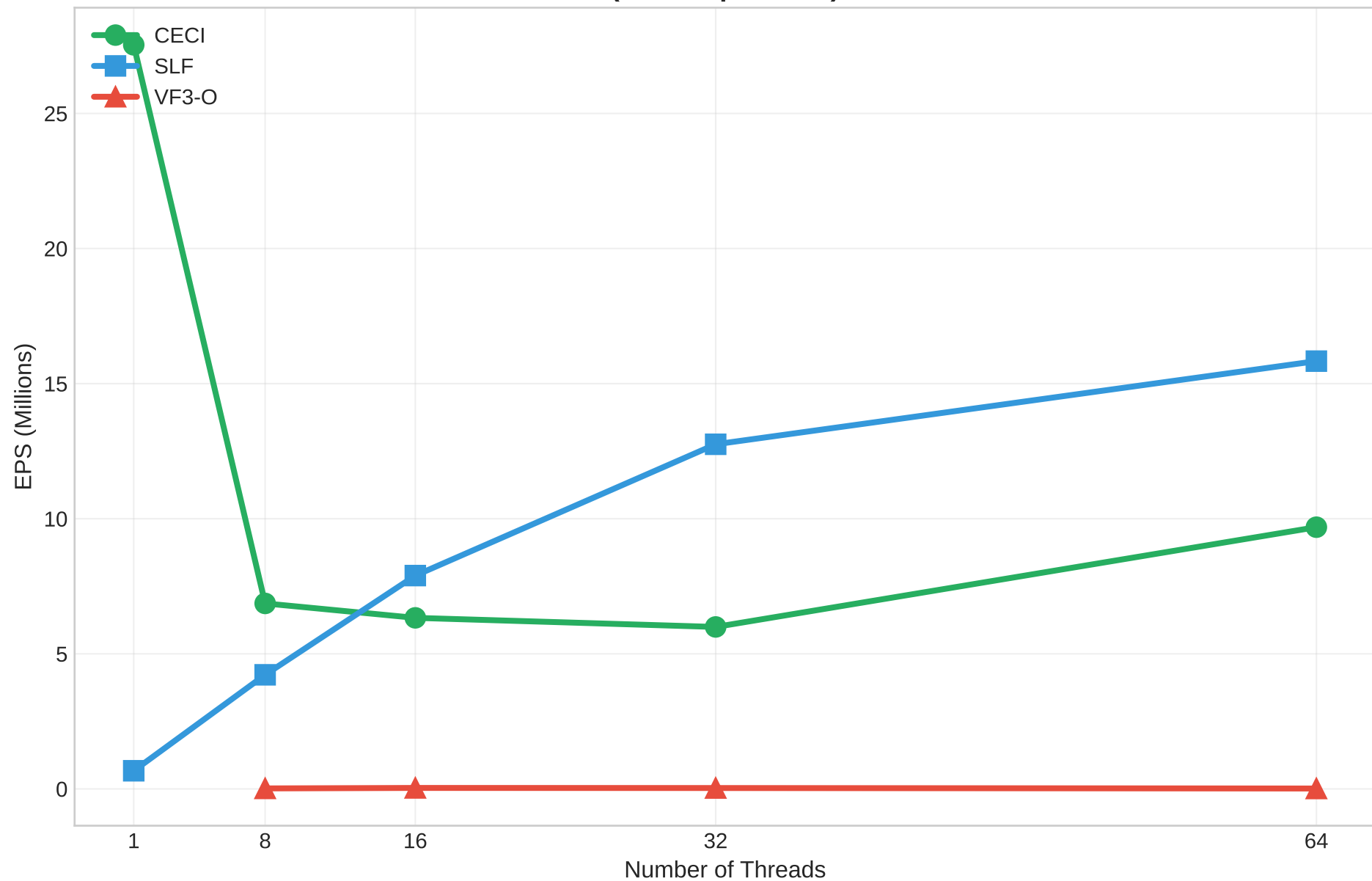
RQ1: Raw Performance vs Thread Count (DBLP Sparse 8v)
