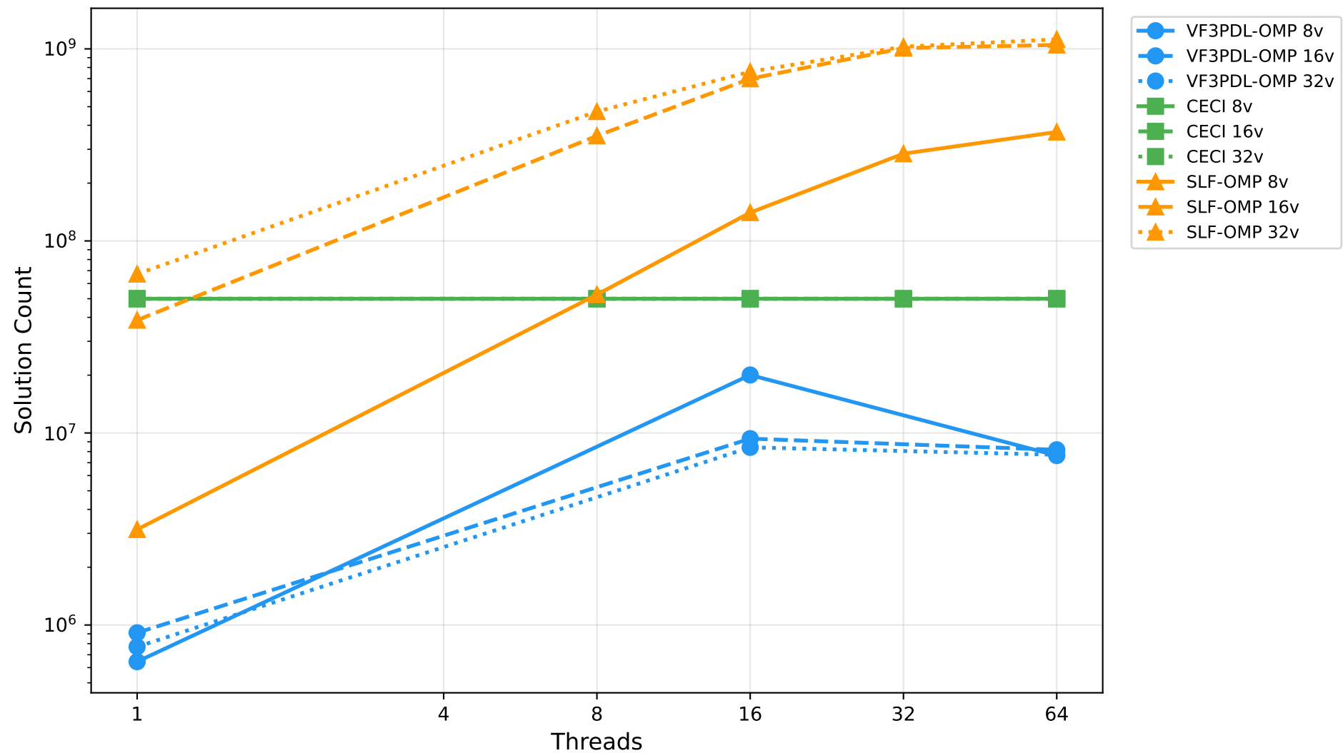
DBLP - Dense Solution Counts
