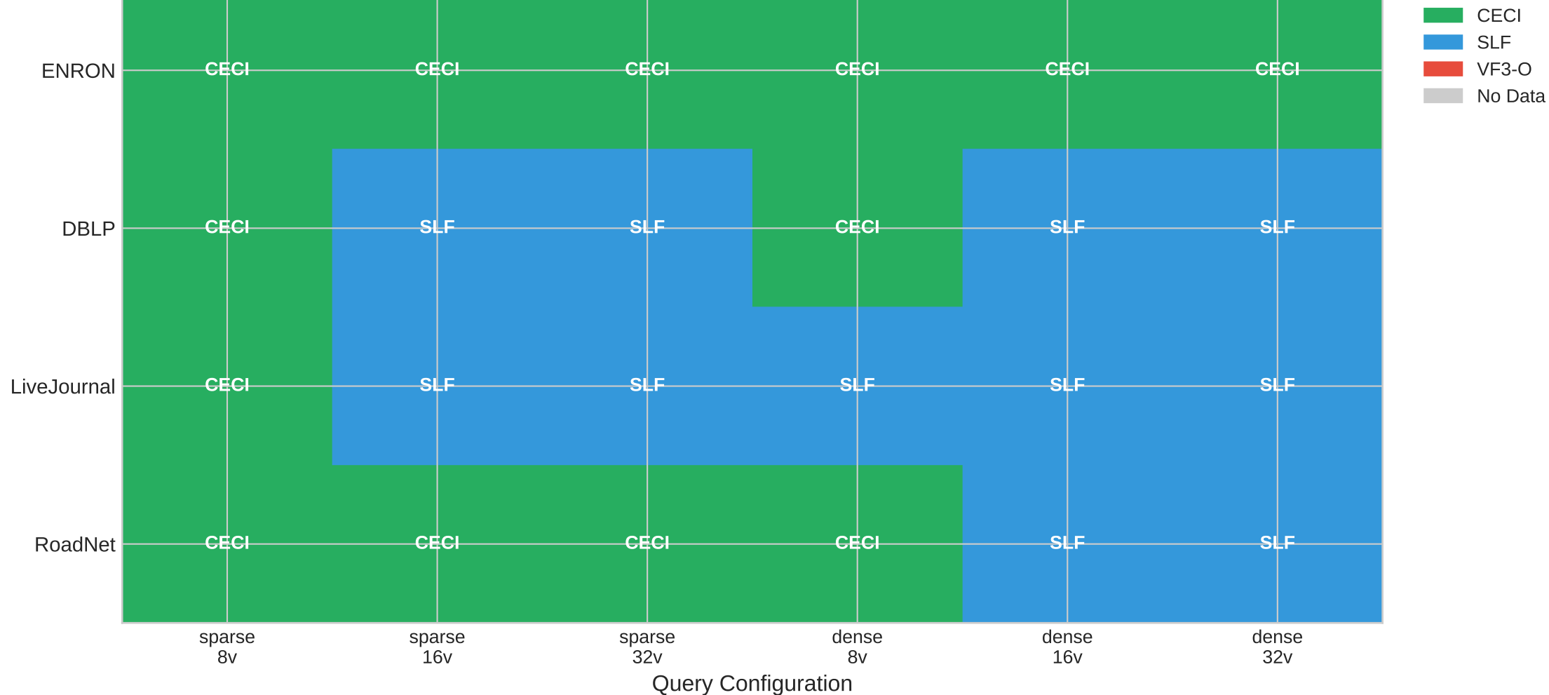
RQ2: Best Algorithm by Dataset and Query Type (CECI dominates small graphs, SLF dominates large graphs)
