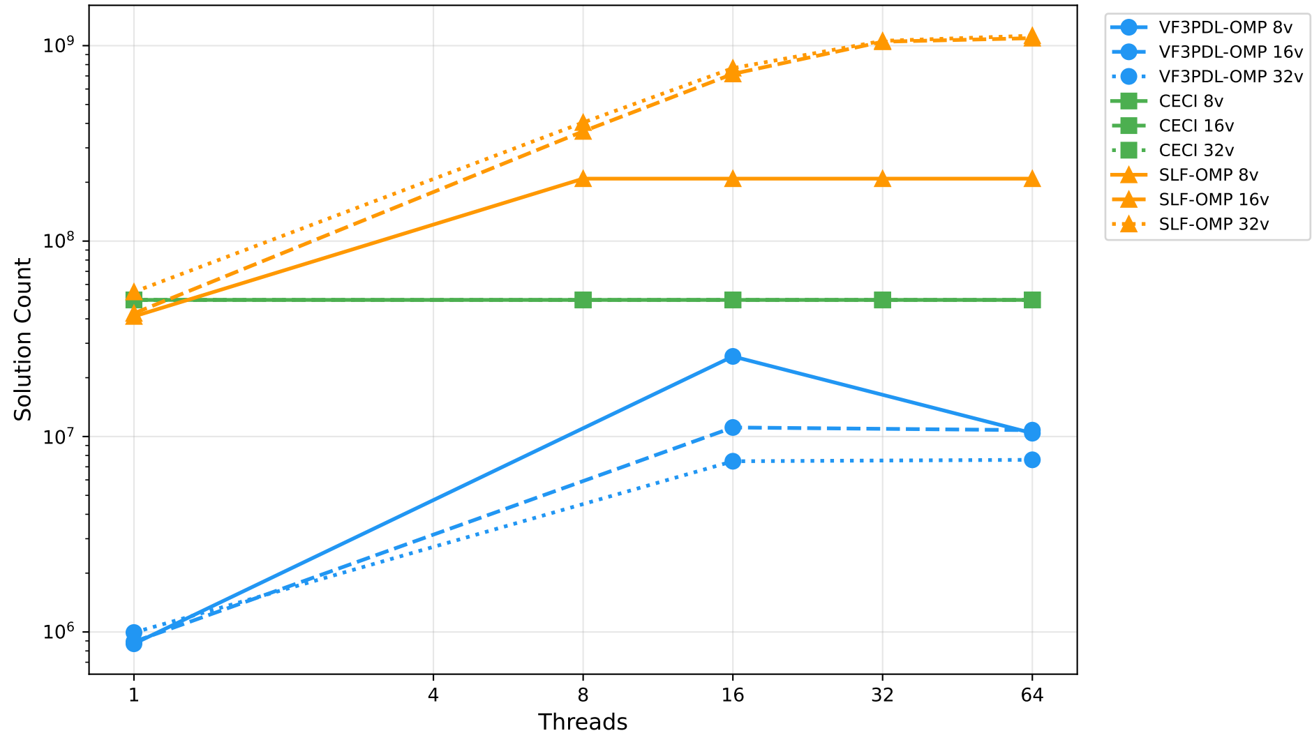
DBLP - Sparse Solution Counts
