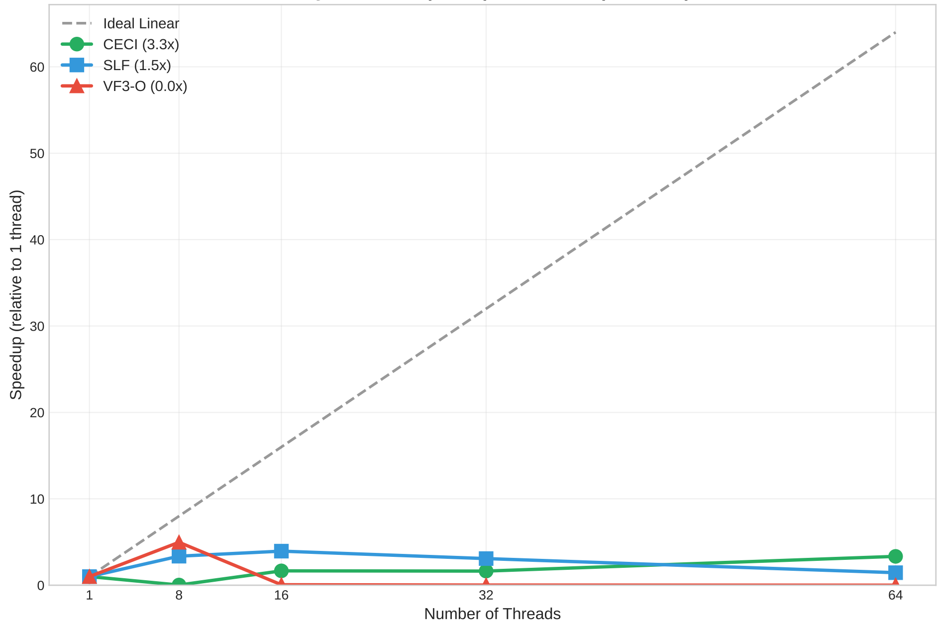
RQ1: Parallel Speedup on ENRON (dense 8v)
