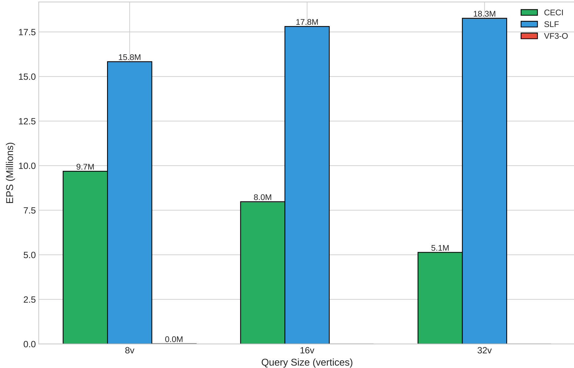
RQ3: Query Size Effect on DBLP (Sparse, 64 Threads) Larger queries = exponentially harder
