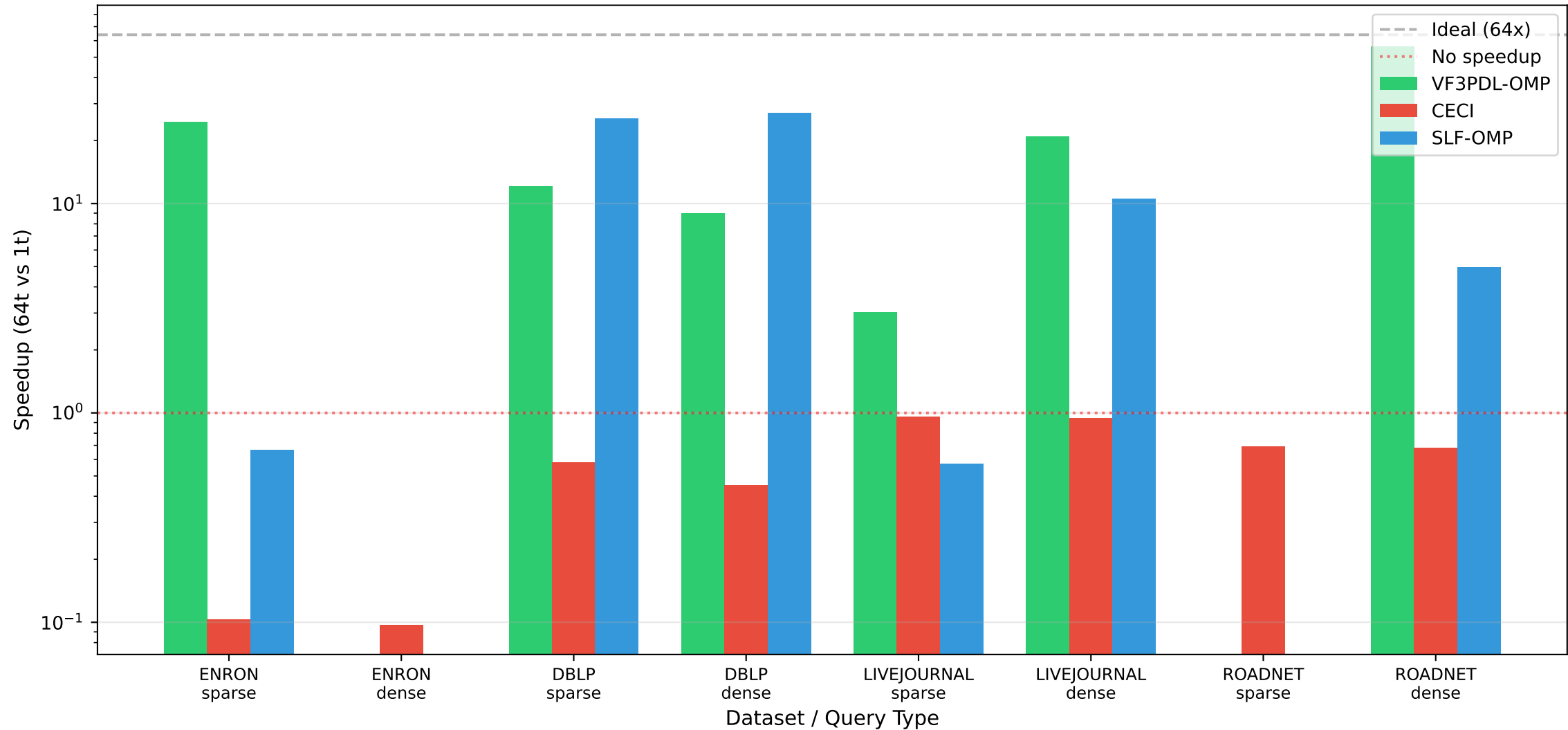
RQ1: Parallel Speedup at 64 Threads
