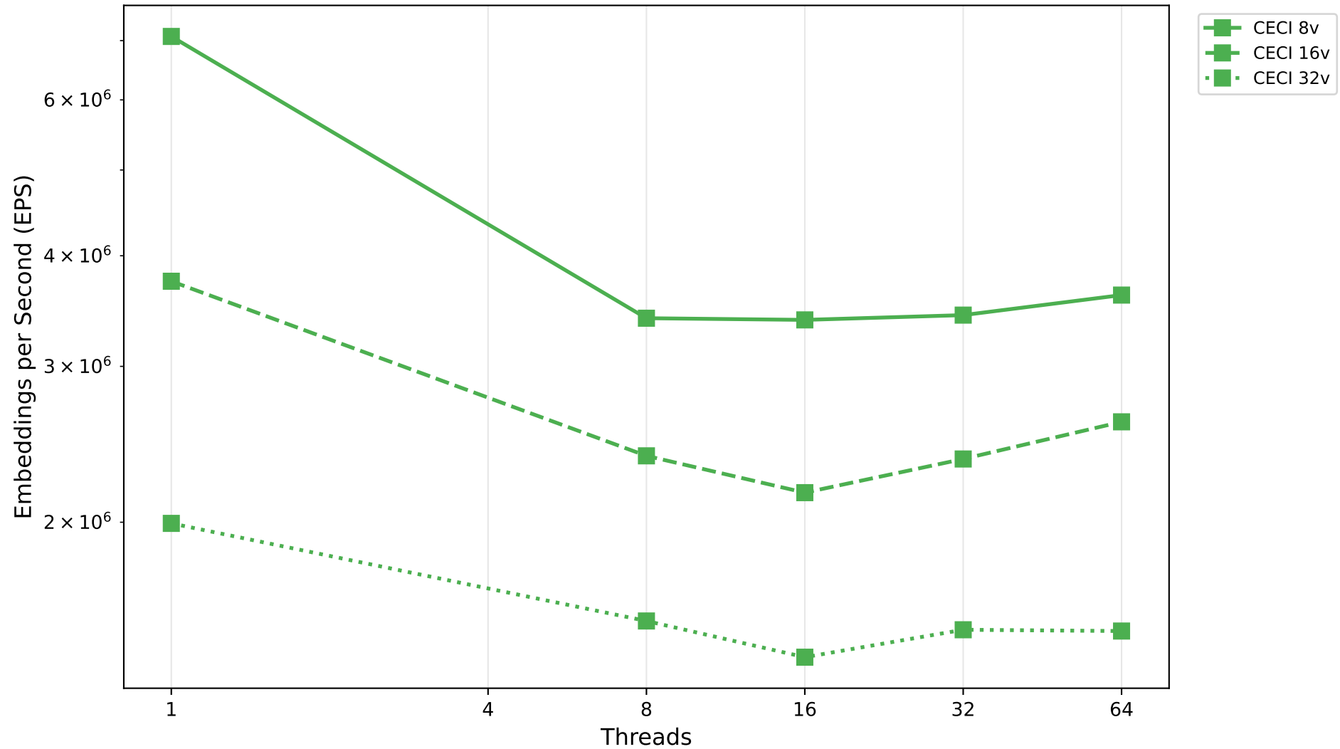
ROADNET - Sparse Queries
