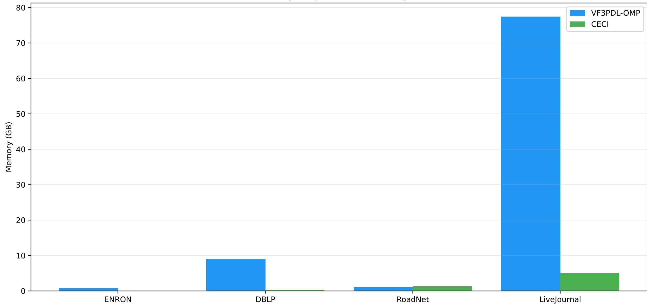
RQ3: Memory Usage @ 64 Threads (Sparse 8v)
