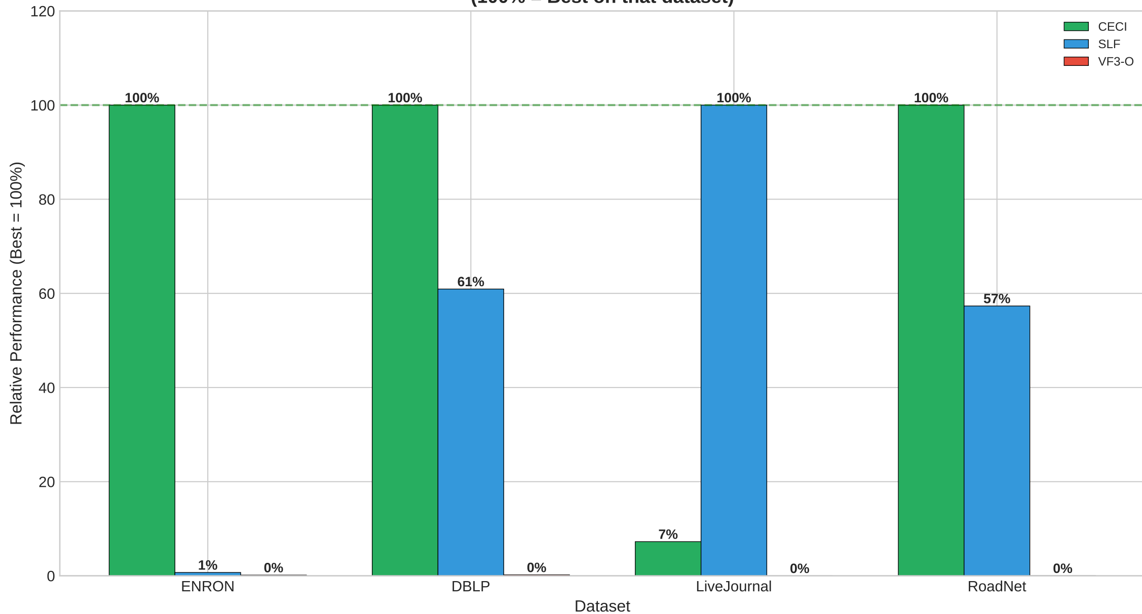
RQ2: Normalized Algorithm Performance (100% = Best on that dataset)
