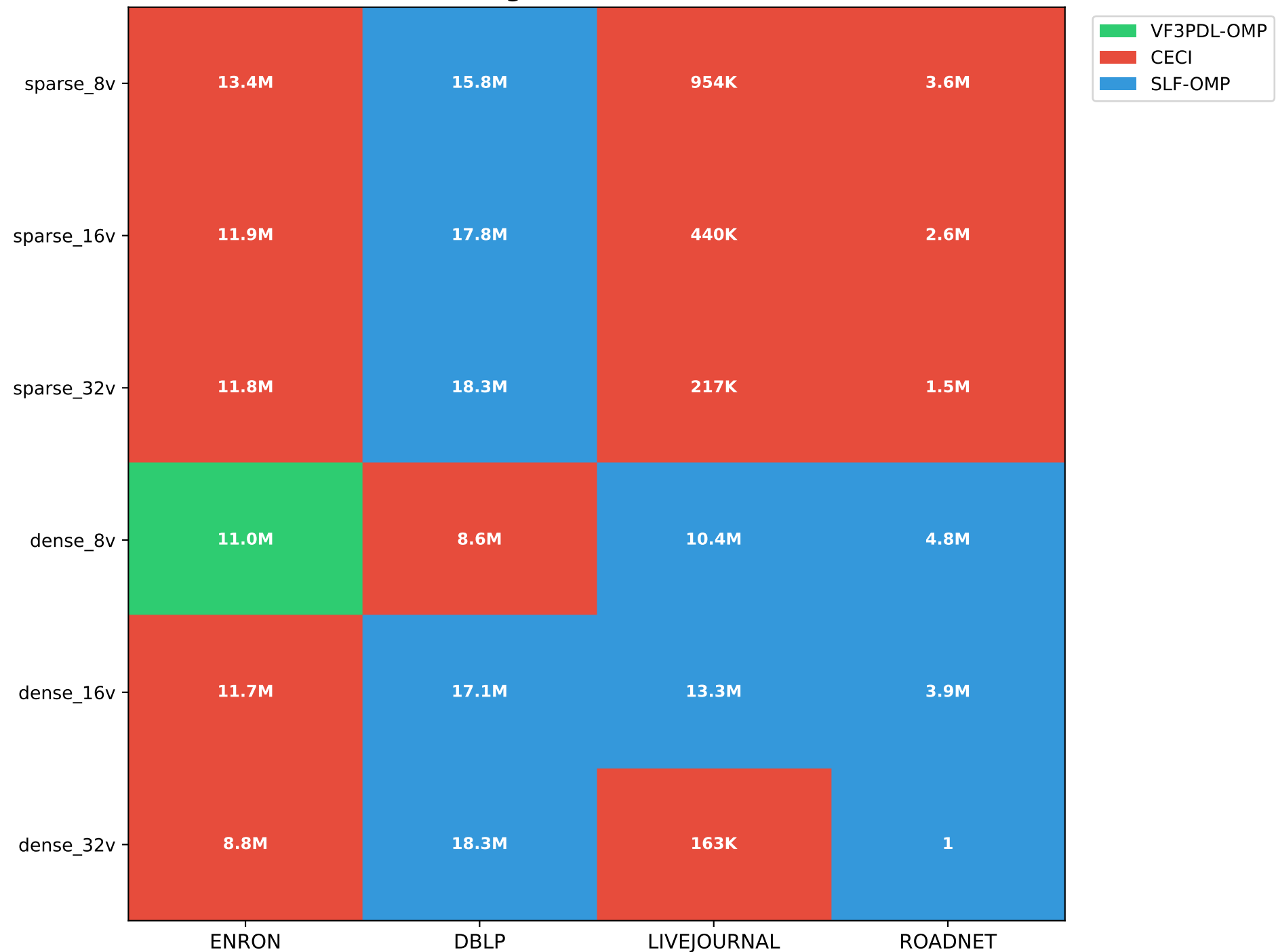
RQ2: Winner by Configuration (@ 64 threads) Color = Best Algorithm, Number = Best EPS
