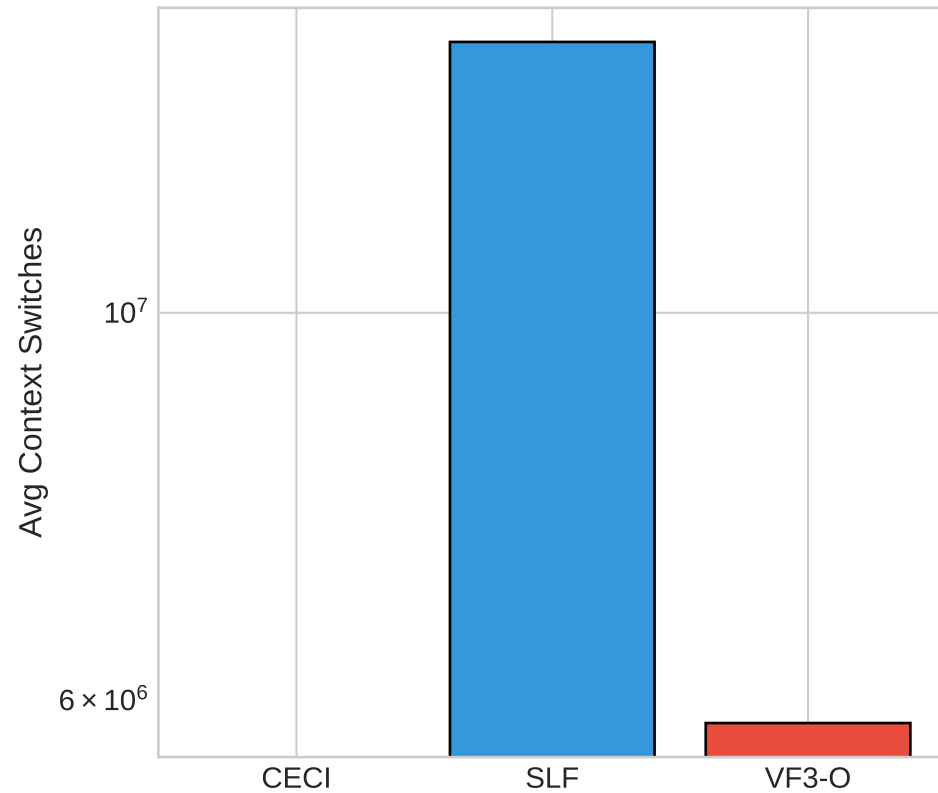
Scheduling Overhead
