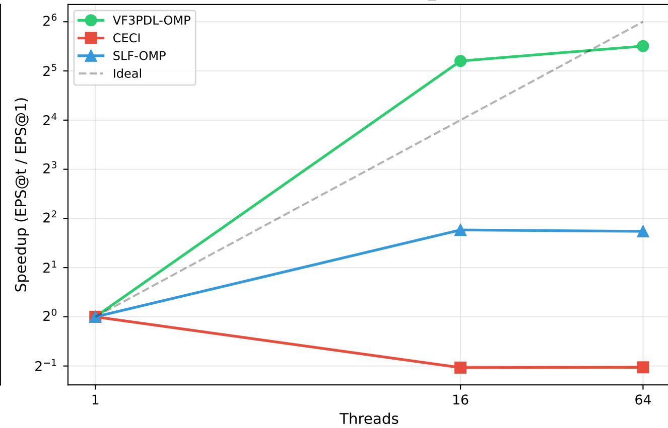
ROADNET (dense_8v)
