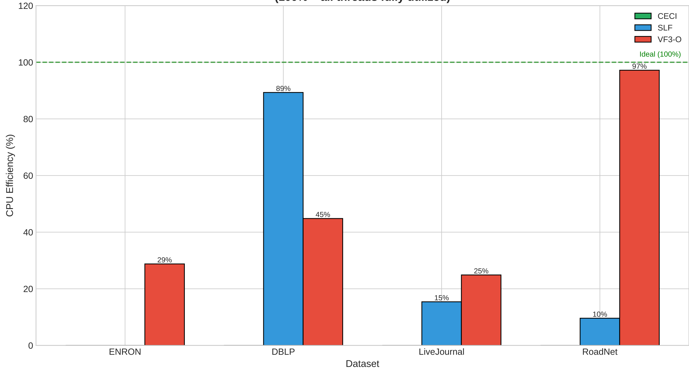
RQ3: CPU Utilization Efficiency at 64 Threads (100% = all threads fully utilized)
