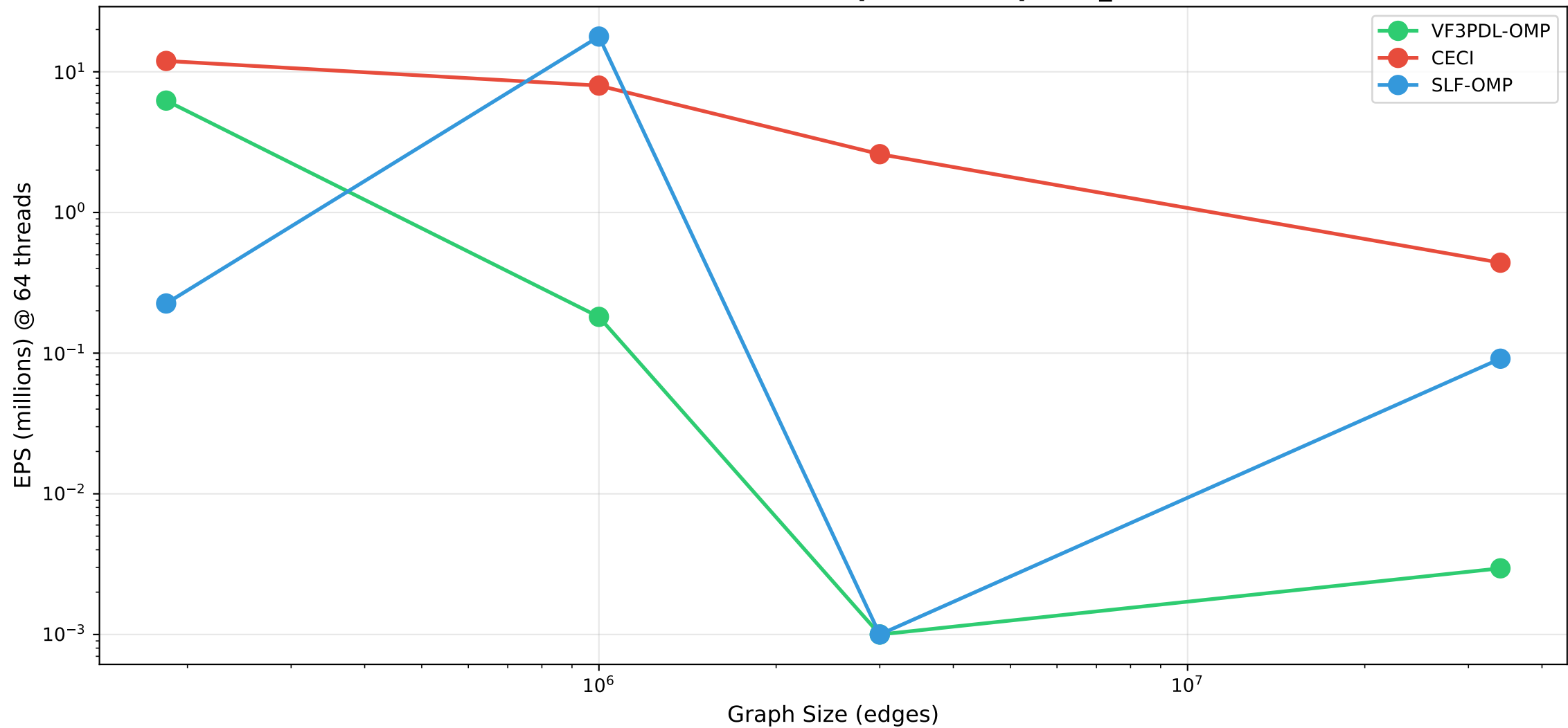
RQ2: Performance vs Graph Scale (sparse_16v)
