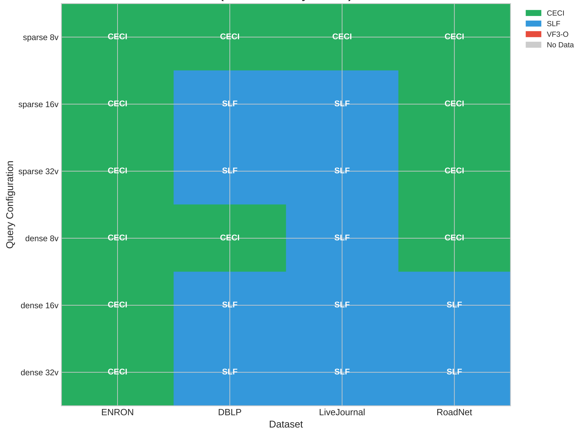
RQ2: Which Algorithm Wins Each Configuration? (Color-coded by winner)
