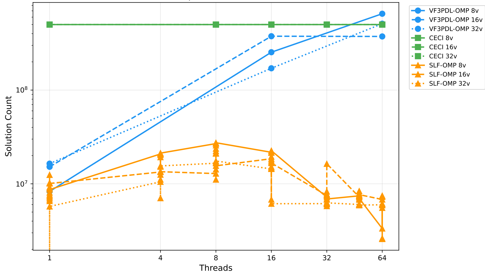
ENRON - Sparse Solution Counts
