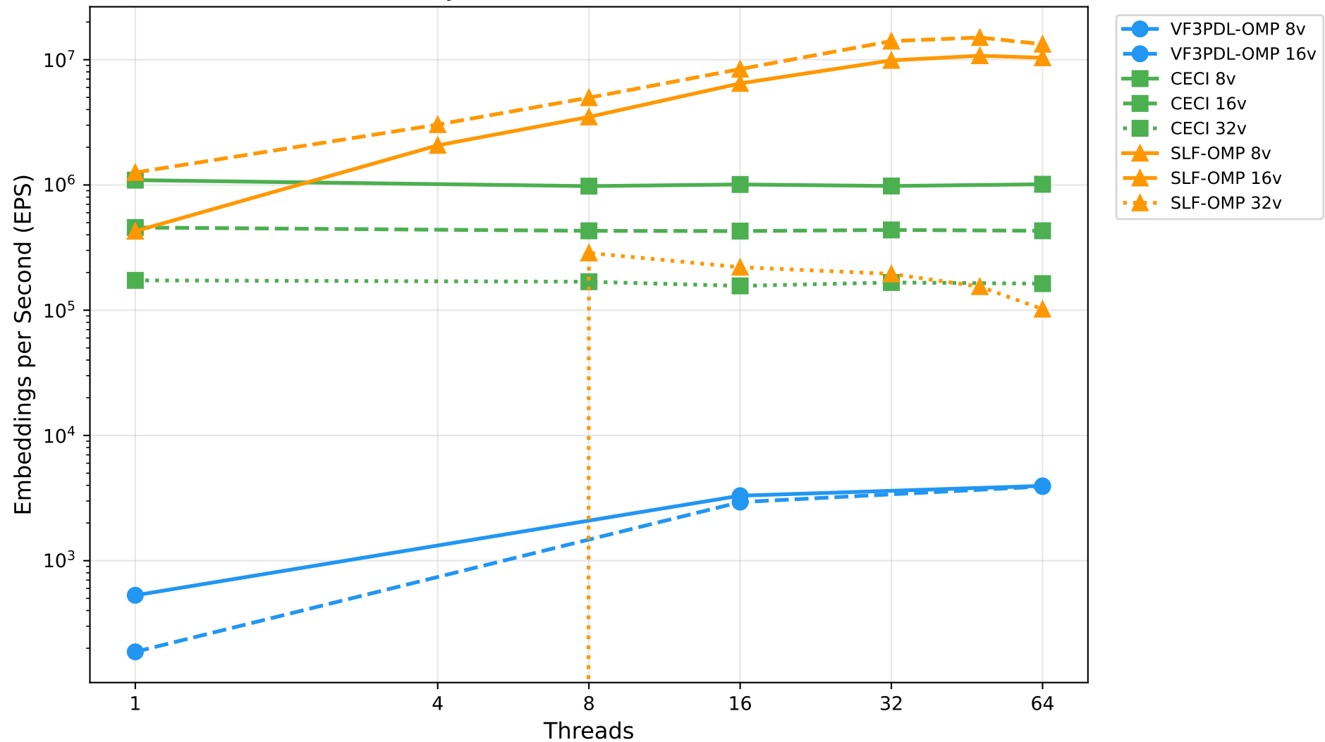
LIVEJOURNAL - Dense Queries
