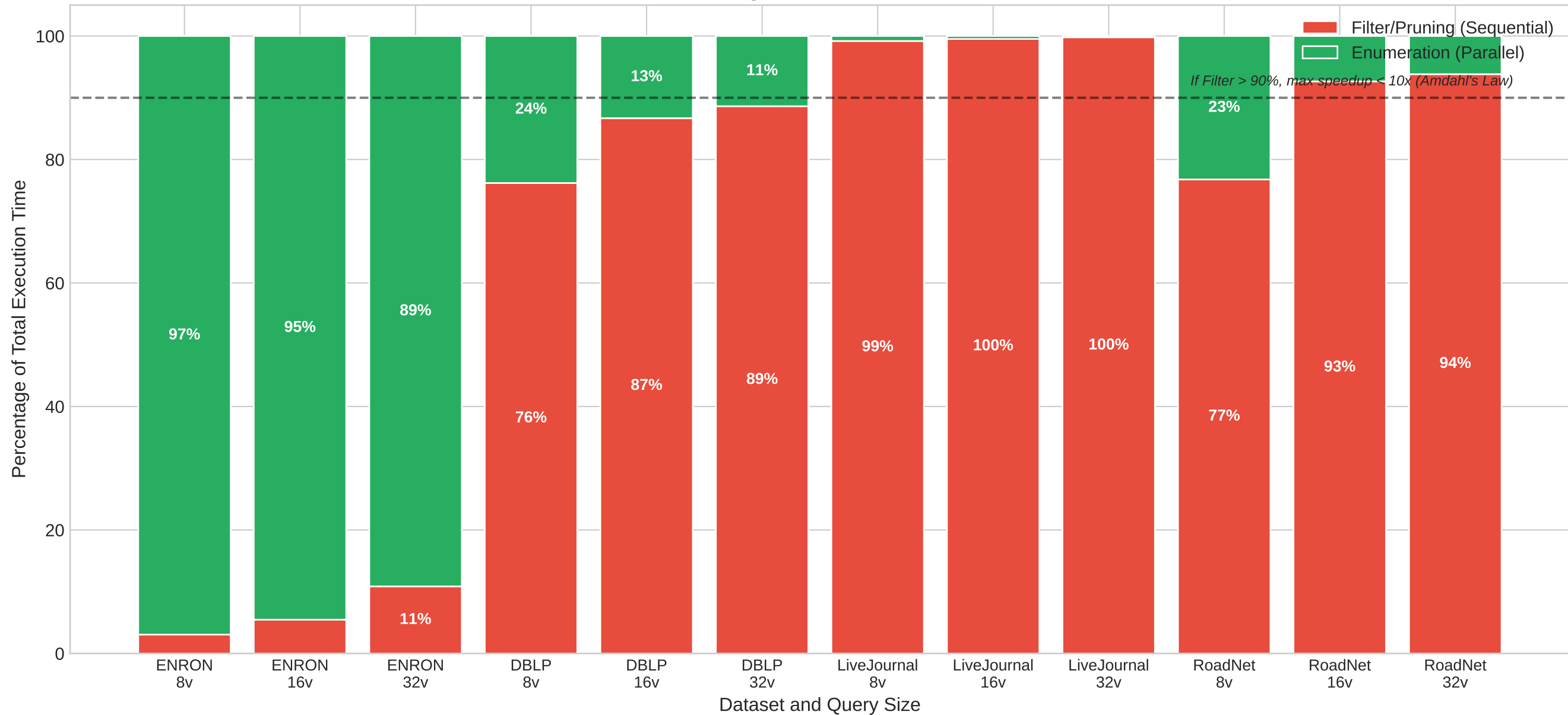
RQ4: Pruning (Filter) Dominates Execution Time CECI Single-Thread Breakdown
