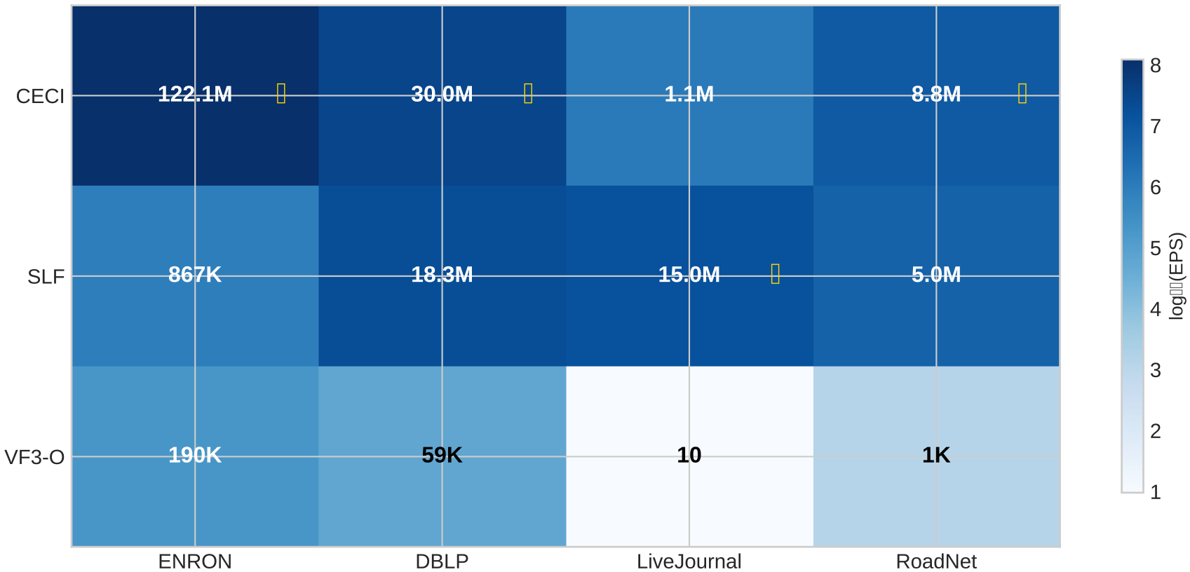
RQ2: Best EPS by Algorithm and Dataset ( \square = Winner)
