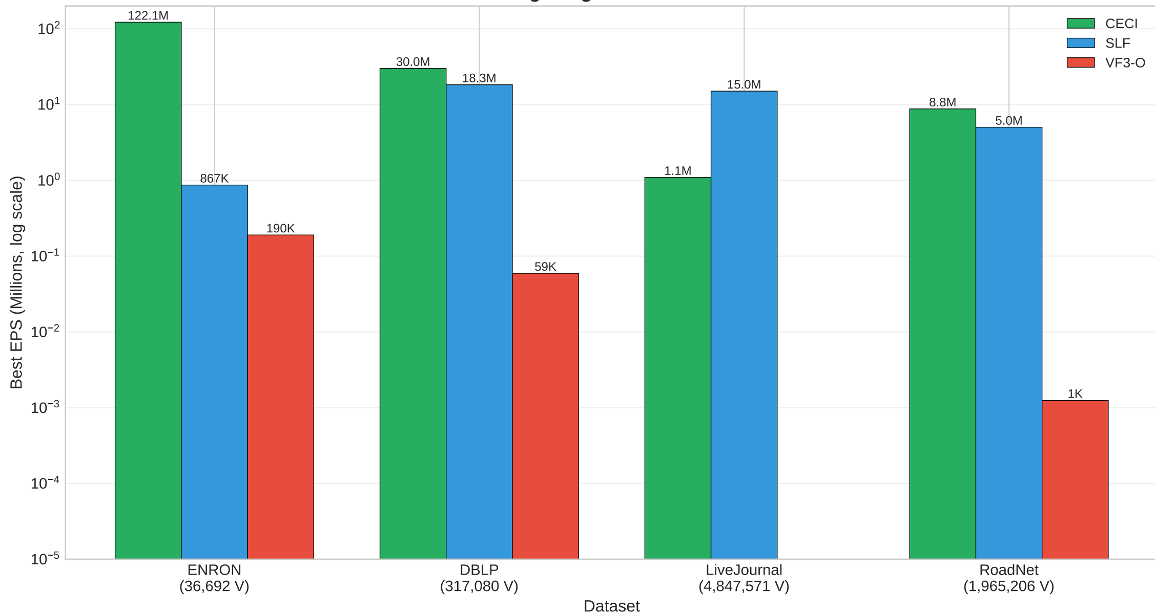
RQ2: Algorithm Performance Varies by Graph Type No Single Algorithm Dominates
