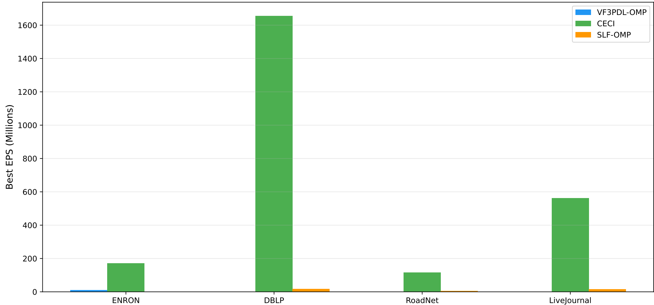
RQ2: Best Performance by Dataset
