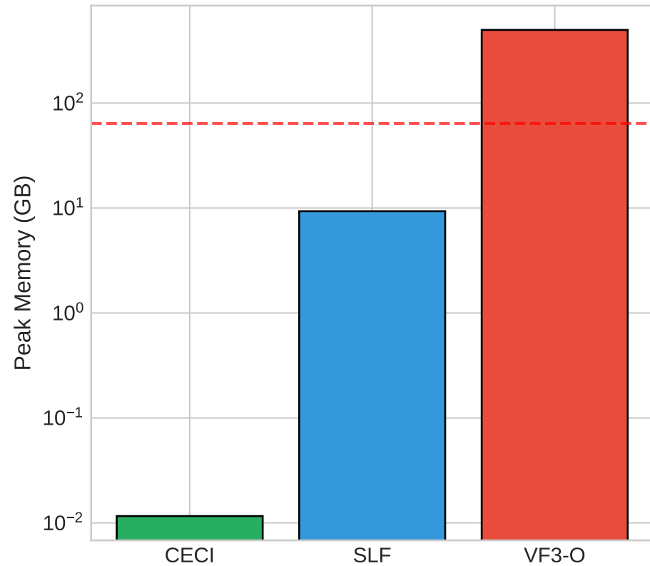
Memory Footprint
