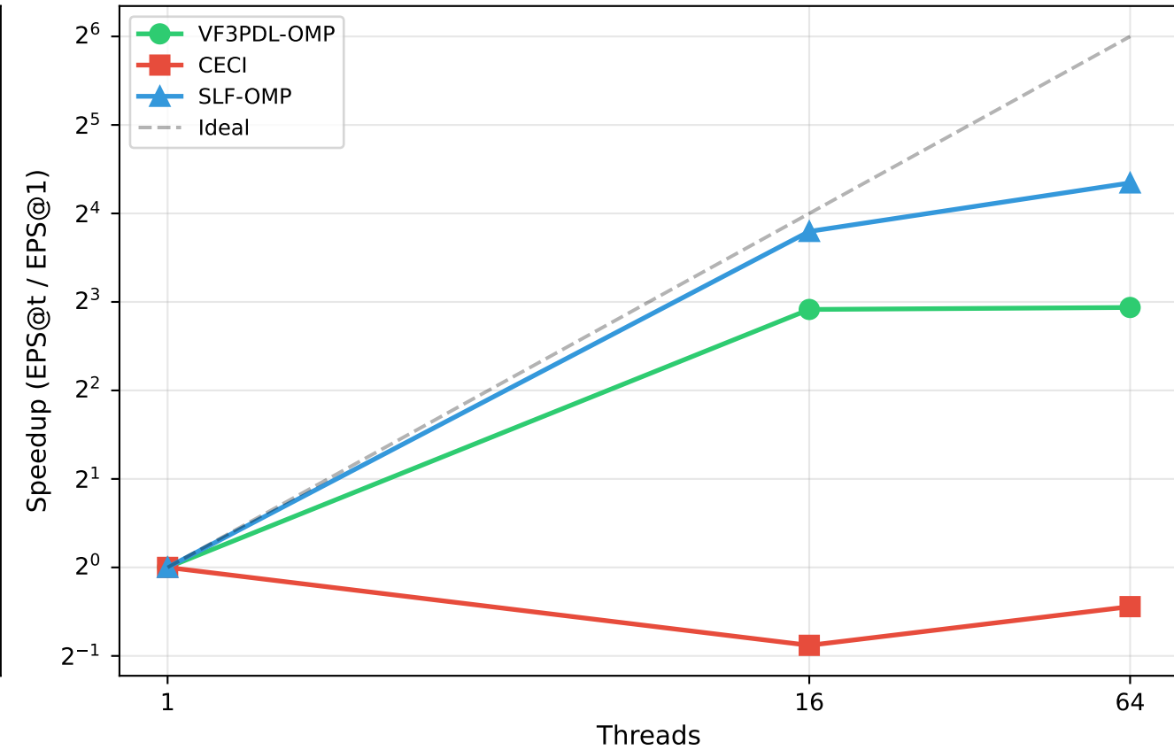
ROADNET (dense_8v)
