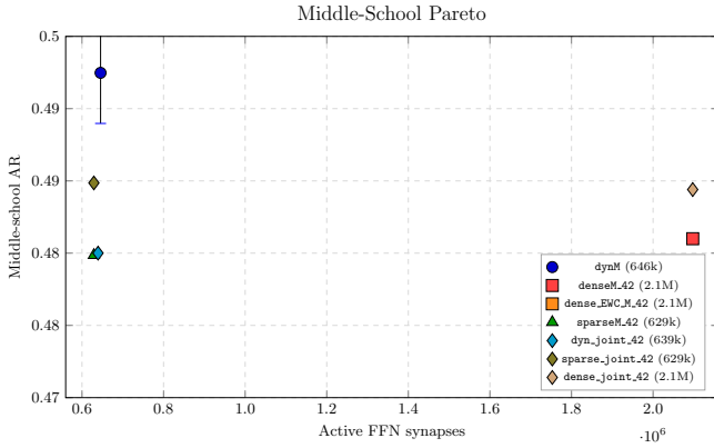
Figure 2: Middle-school-level performance across substrates and protocols. At the middle-school level, dense, dynamic, and static sparse models fall in a narrow AR band despite large differences in active FFN budget. Joint controls are shown as level-slice references under a different exposure regime from sequential CL. Error bars are shown only for the multi-seed DYNCL point; all other controls are single-seed.
