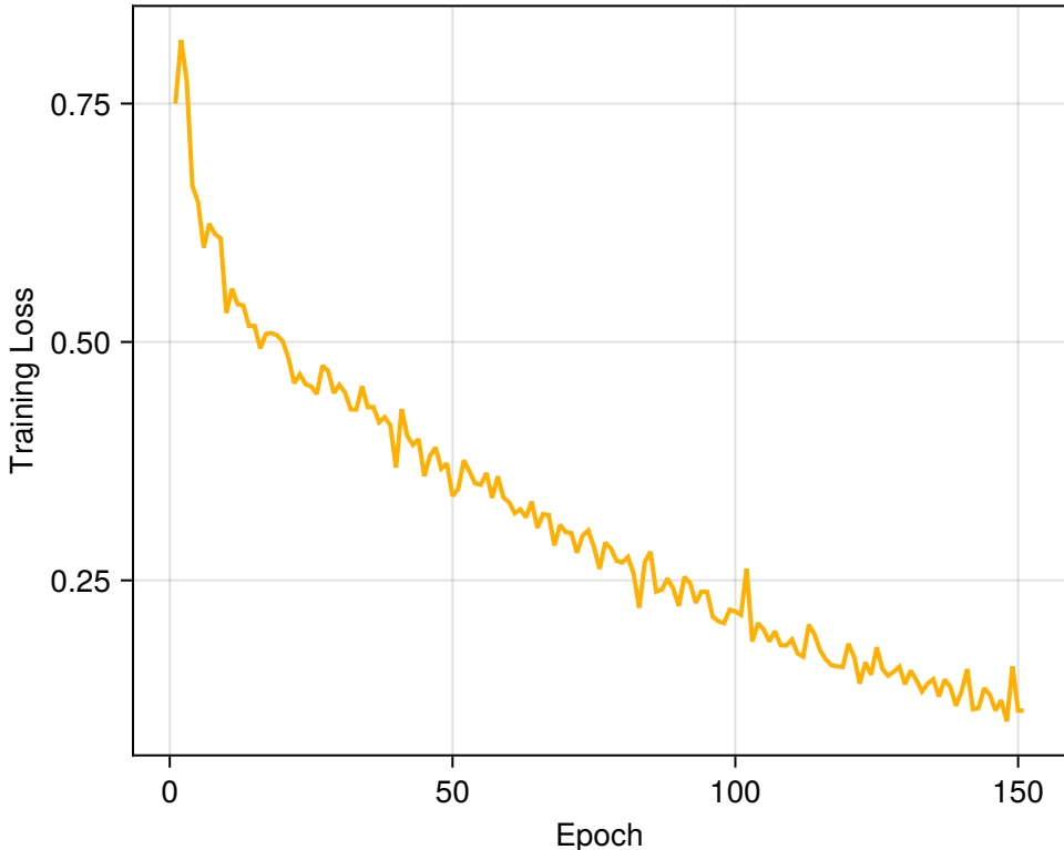
Outer Fold 4
