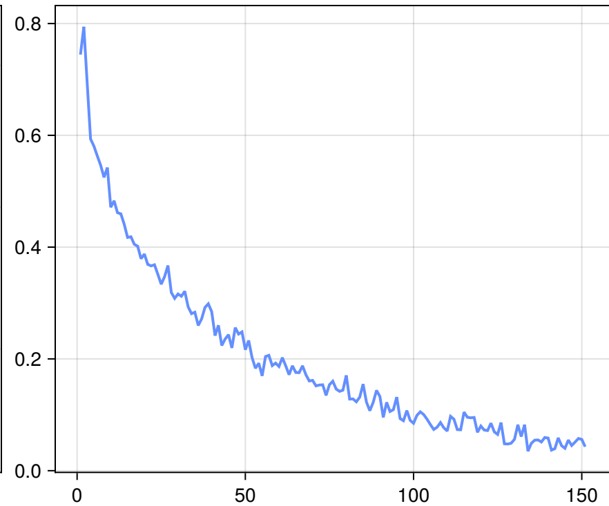
Outer Fold 5
