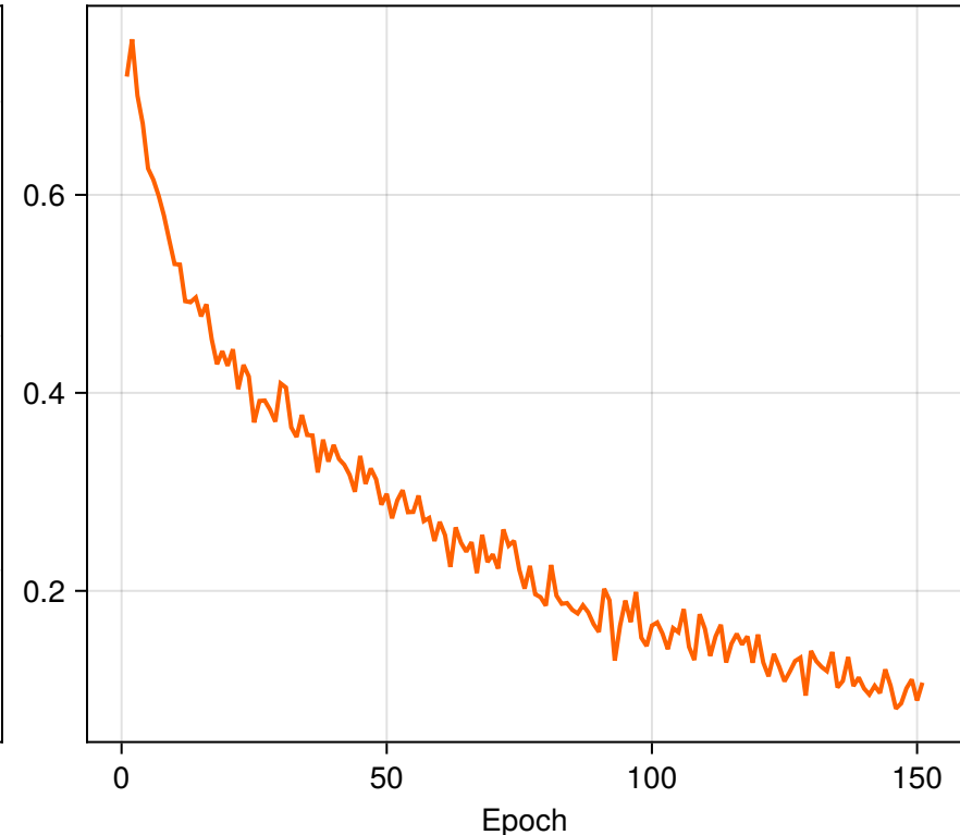
Outer Fold 5
