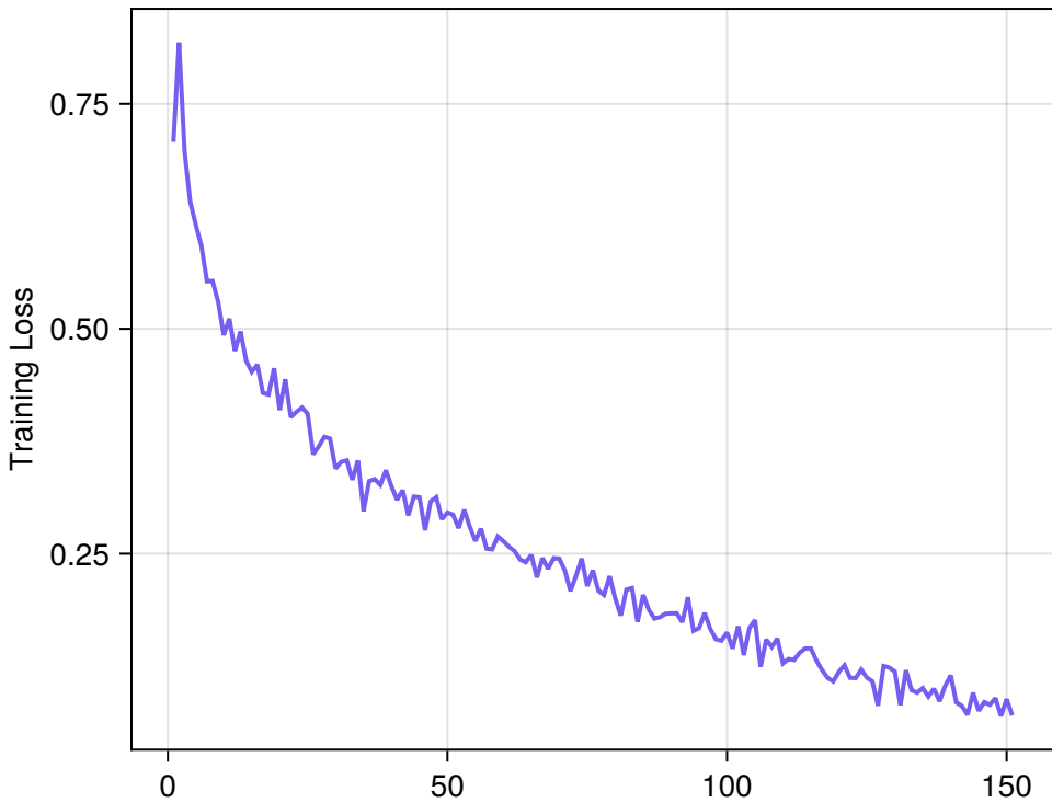
Outer Fold 4
