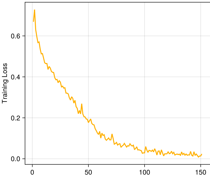
Outer Fold 4
