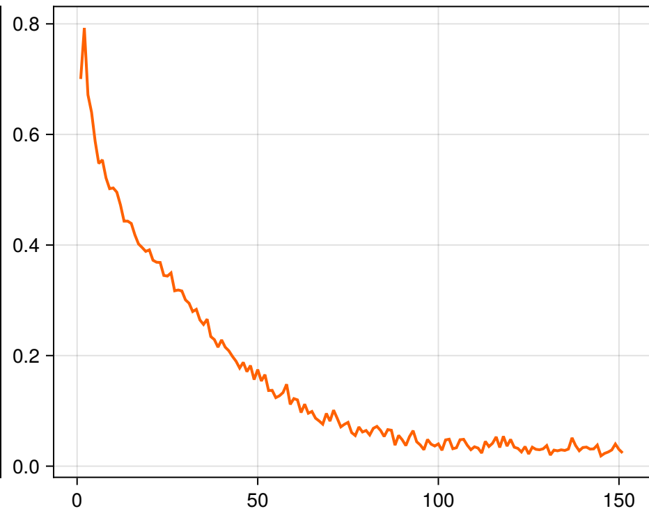
Outer Fold 5
