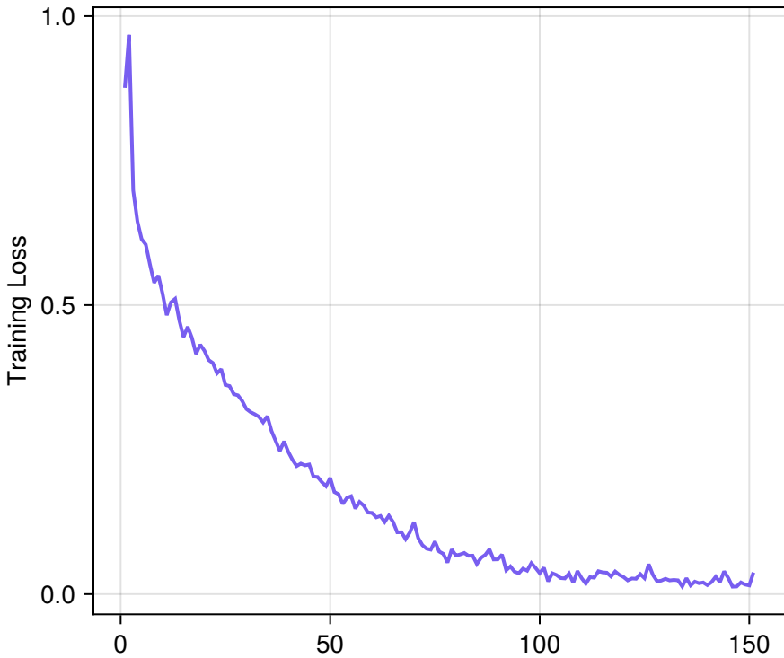
Outer Fold 4
