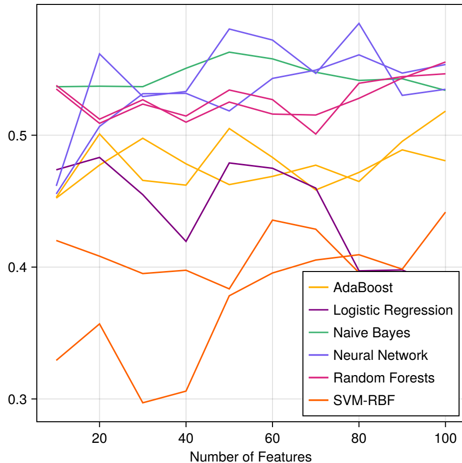
baseline — mRMR
