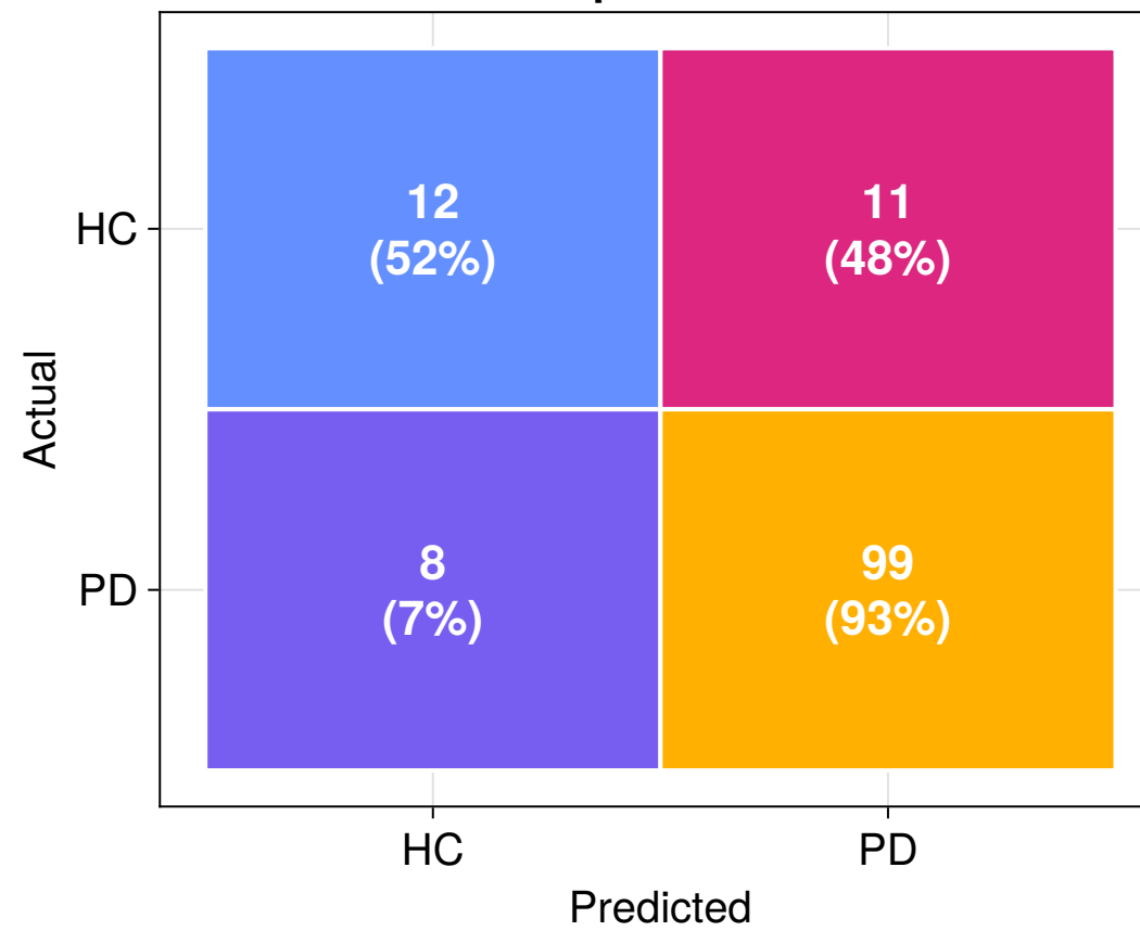
Male-Specific Model
