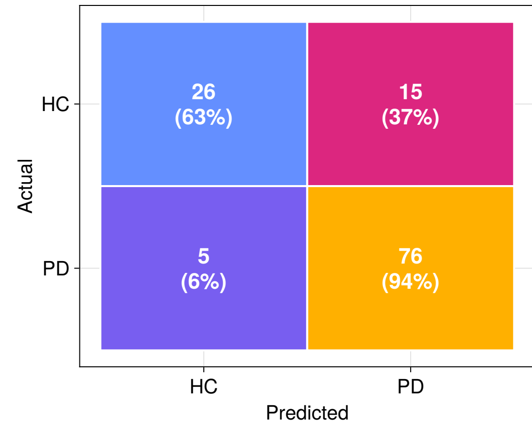
Full Dataset-Female
