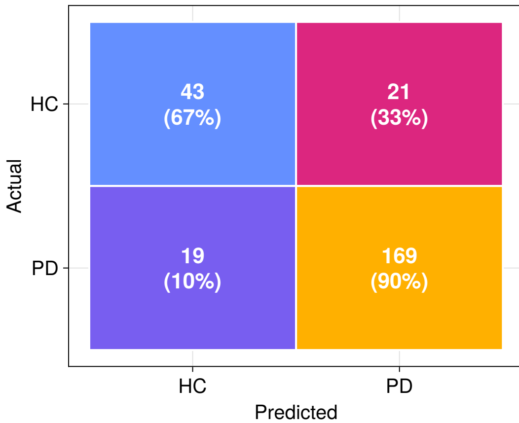
Sex-Aware
