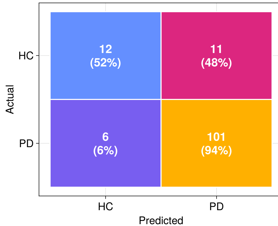
Full Dataset-Male
