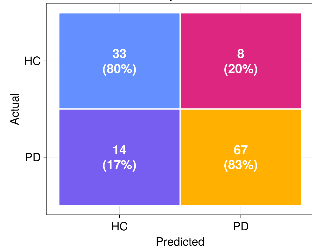
Female-Specific Model
