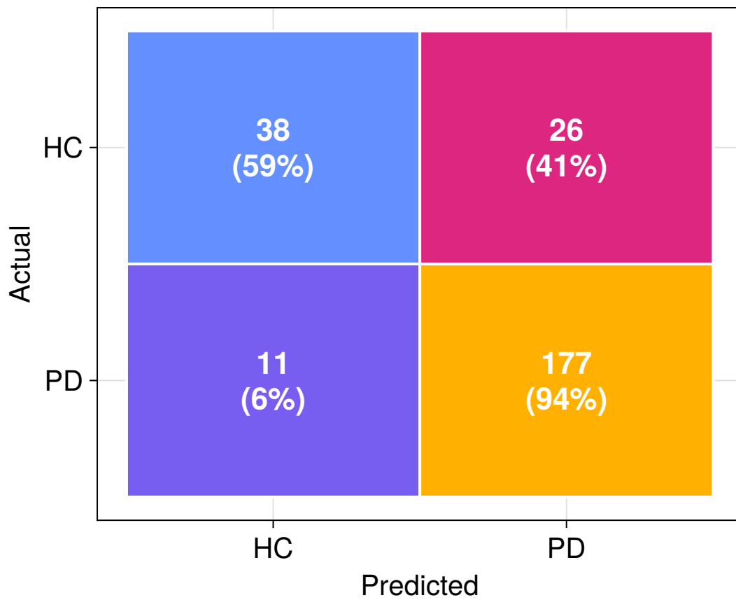
Full Dataset
