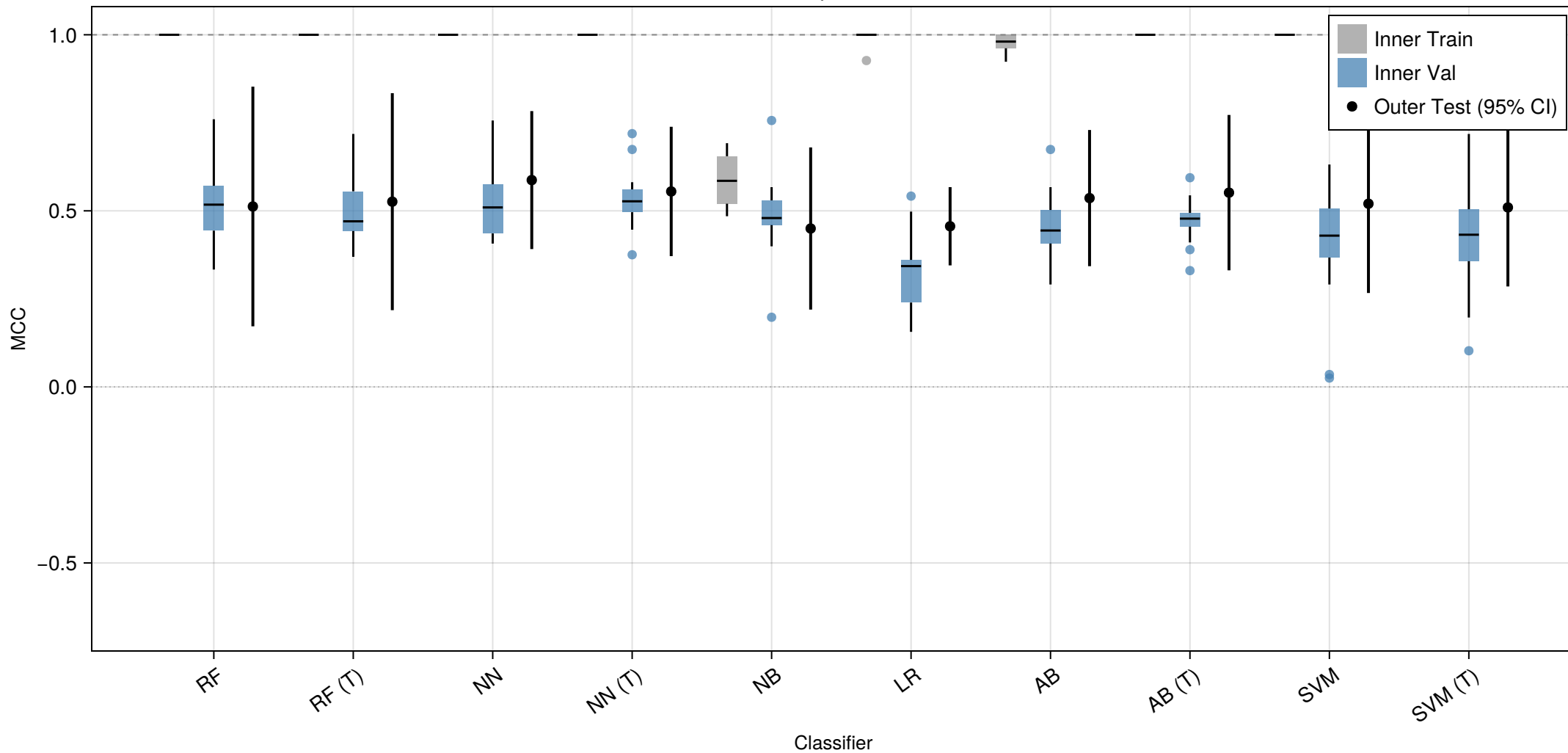
Full Dataset | Boruta, N=100
