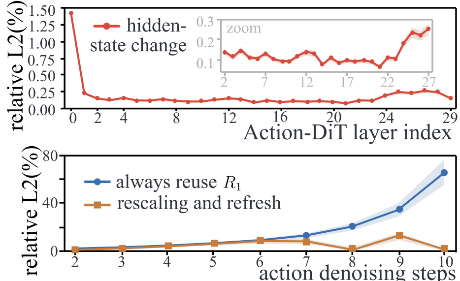
(c) layer state continuity
