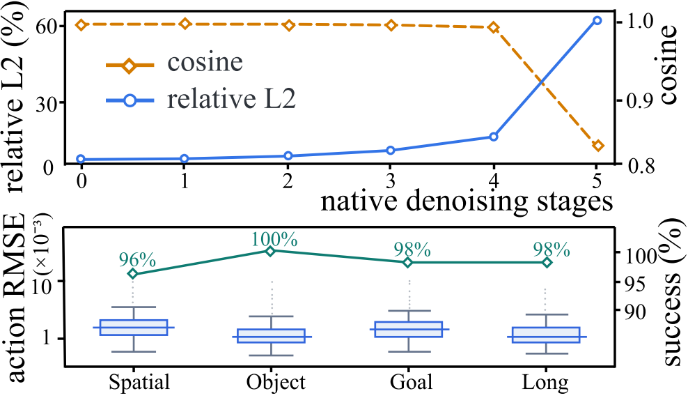
(a) replan state continuity
