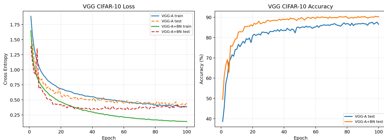
图 6: Training curves for VGG-A and VGG-A+BN. BN improves both convergence and final accuracy.
