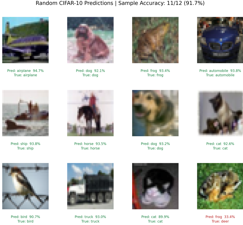
图 2: Qualitative predictions from the Part 1 best checkpoint.
