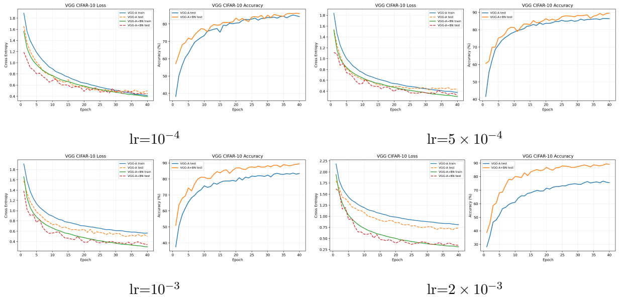
图 4: VGG learning-rate sweep curves. BN keeps the curves stable under larger learning rates.
