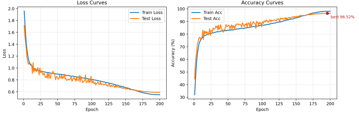
图 1: Training and test curves of the Part 1 best-checkpoint run.
