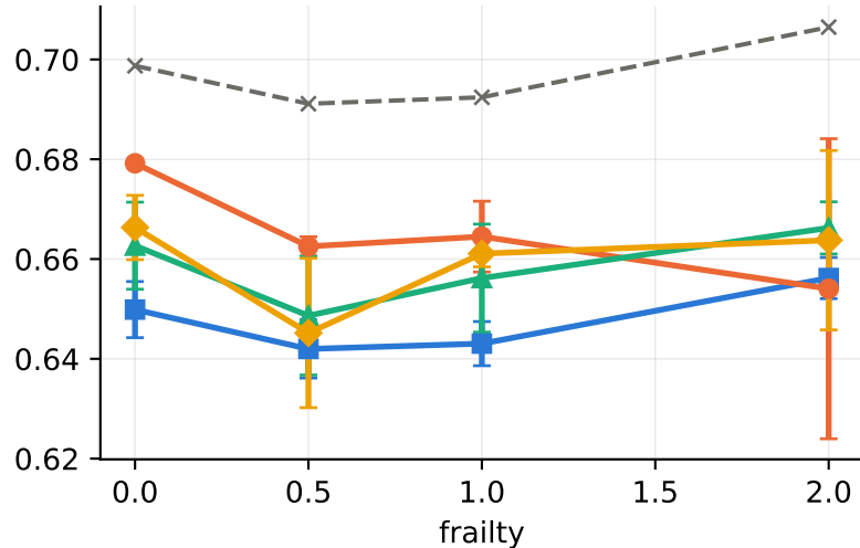
Within-subject C \uparrow
