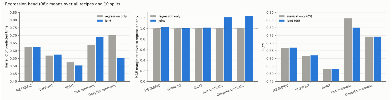
Figure 5: Means over all recipes and splits. Left: Harrell’s C of the predicted time; middle: MAE relative to the regression-only models; right: C_{td} of survival-only (notebook 05) and joint models.
