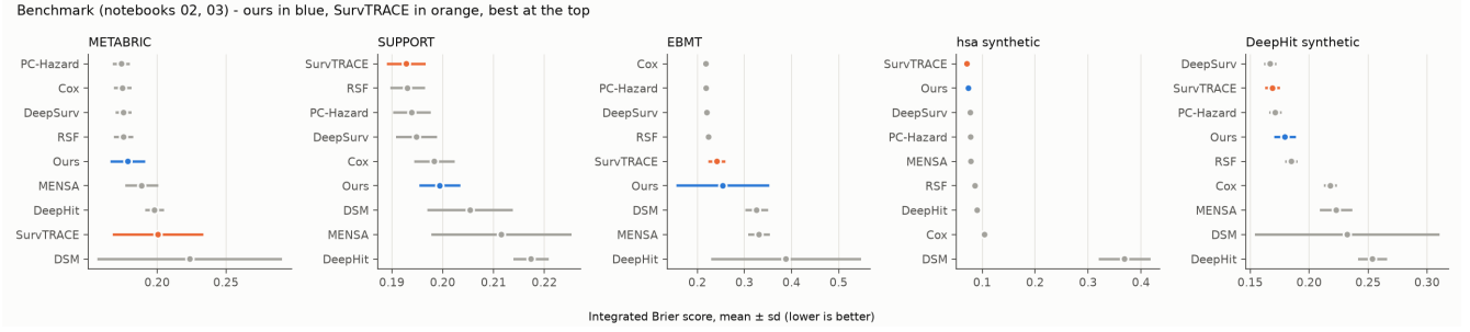
Figure 1: Integrated Brier score per dataset; ours in blue, SurvTRACE in orange.
