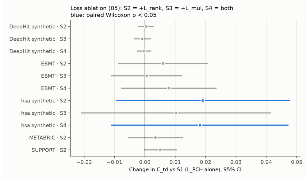
Figure 2: Change in C_{td} against S1 with 95% confidence intervals; blue: paired Wilcoxon p < 0.05 .
