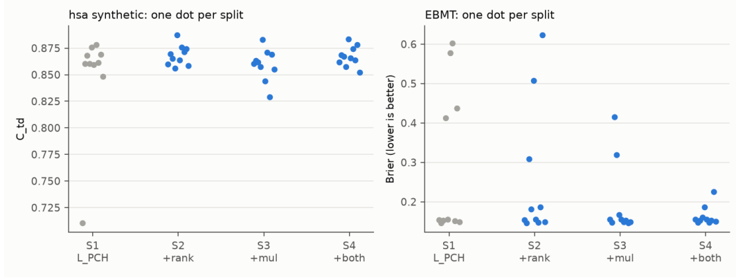
Figure 2: Every split of each loss variant. Left: C_{td} on hsa synthetic. Right: Brier score on EBMT. With L_{PCH} alone (S1) some splits fail; with L_{rank} + L_{mul} (S4) none do.
