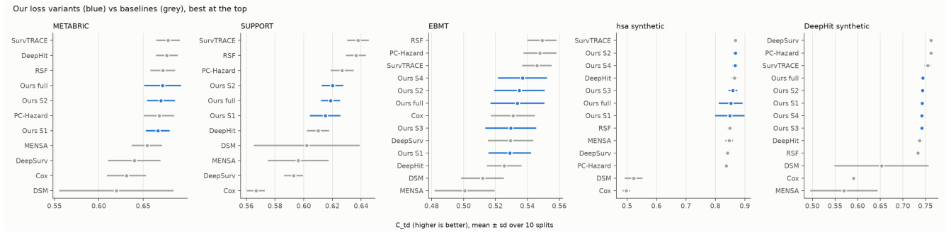
Figure 1: C_{td} of our variants (blue) and the baselines (grey), best at the top of each panel.
