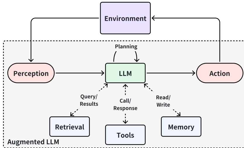
FIGURE 2.2: Augmented LLM-based agentic system [2].
