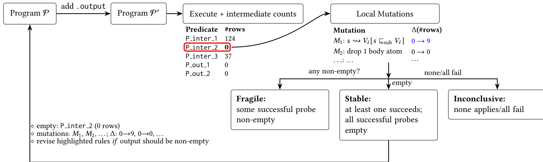
FIGURE 5.3: Intermediate-rule mutation and feedback.
