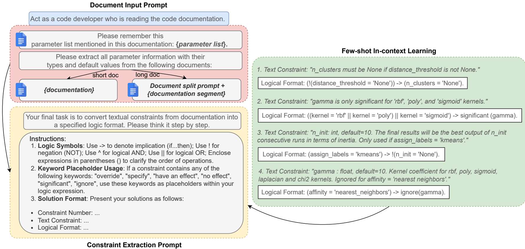
FIGURE 4.7: Prompt structure for constraint extraction.
