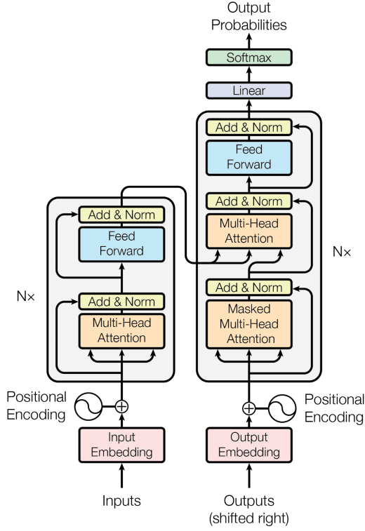
FIGURE 2.1: The Transformer model architecture [1].
