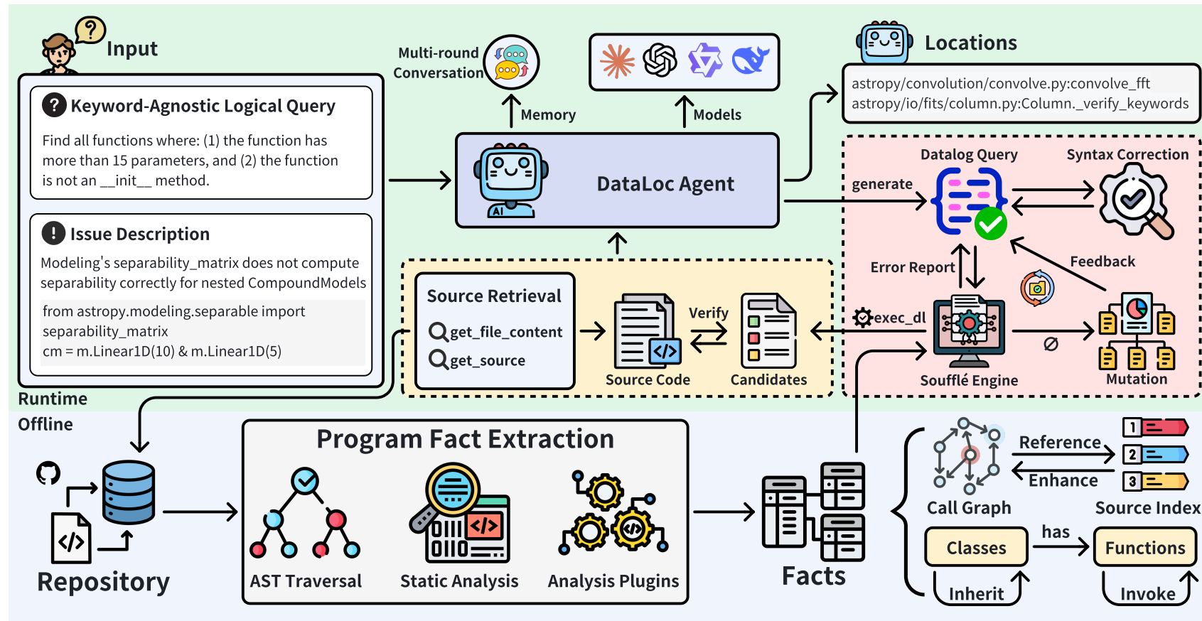
FIGURE 5.2: Overview of the DATALOC framework.
