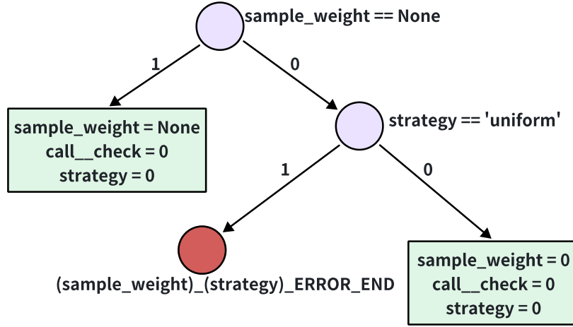
FIGURE 4.6: Path constraints corresponding to the code in Figure 4.5.
