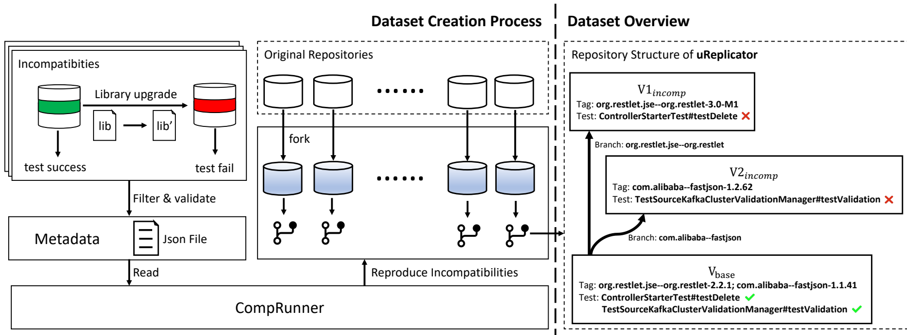
FIGURE 3.2: The architecture of COMPSUITE.
