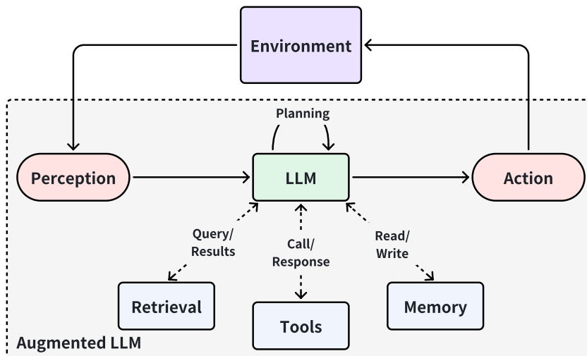
FIGURE 2.2: Augmented LLM-based agentic system.
