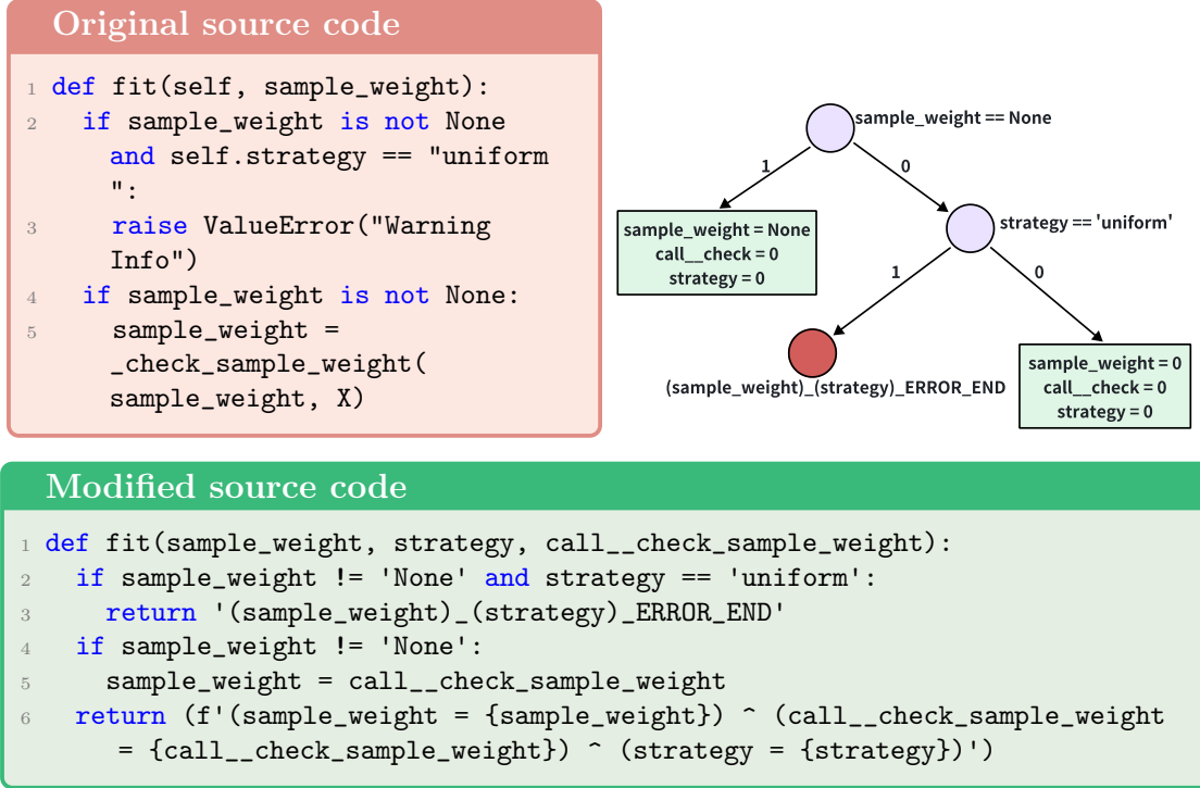
FIGURE 4.5: Extracting constraint from code
