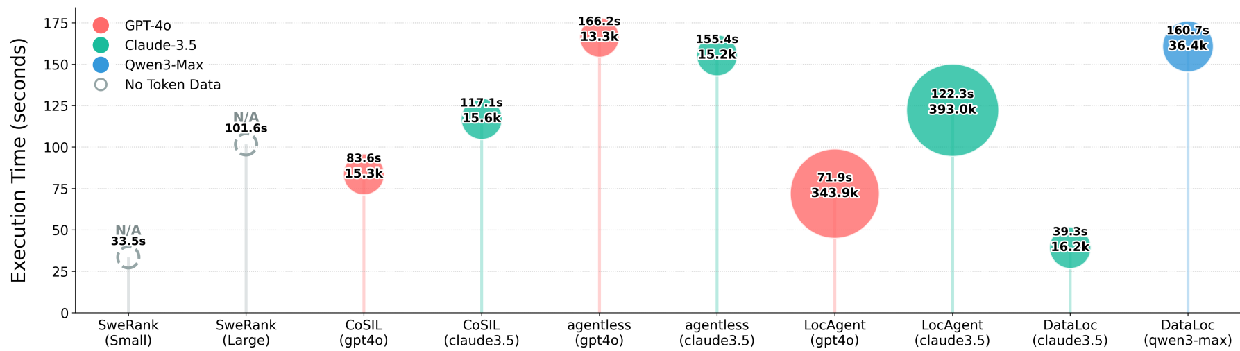
FIGURE 5.4: Average execution time and token consumption of KA-LOGICQUERY.
