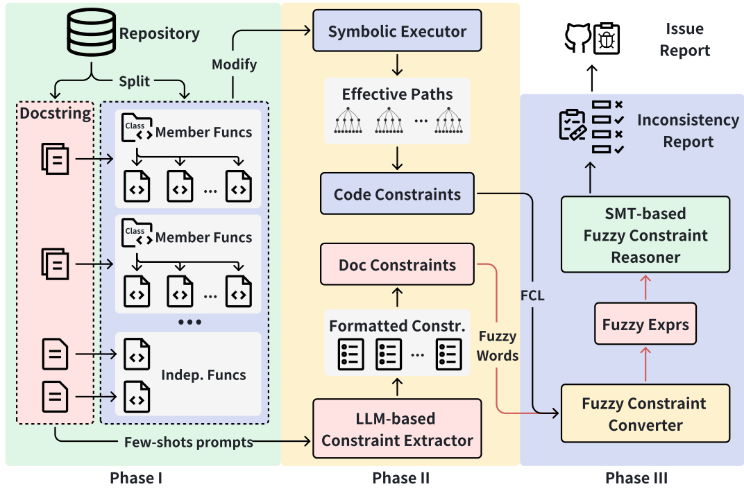
FIGURE 4.3: The architectural overview of MPCHECKER.
