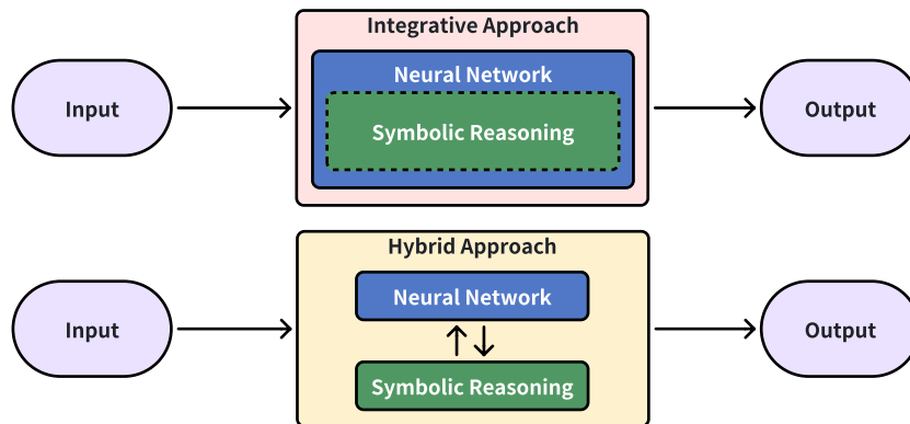
FIGURE 2.2: Integrative and hybrid neurosymbolic approaches.
