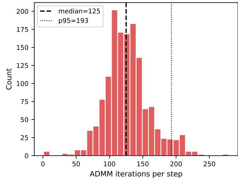
ADMM iteration distribution
