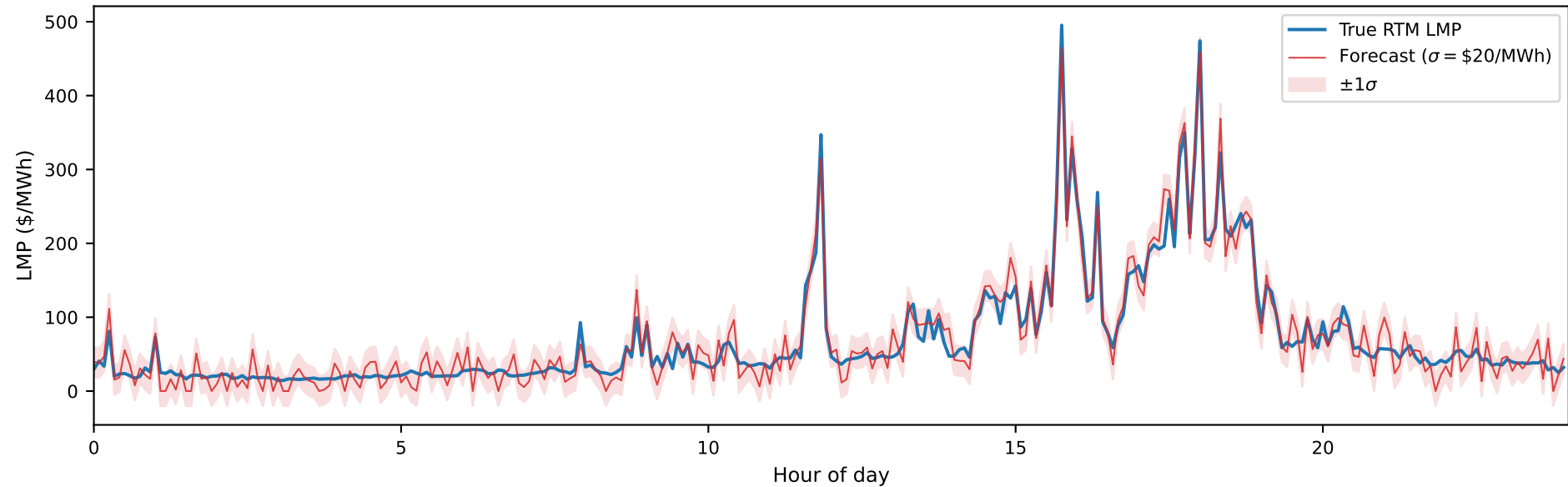
RTM LMP: True vs Forecast — Day 1 (2024-07-08)
