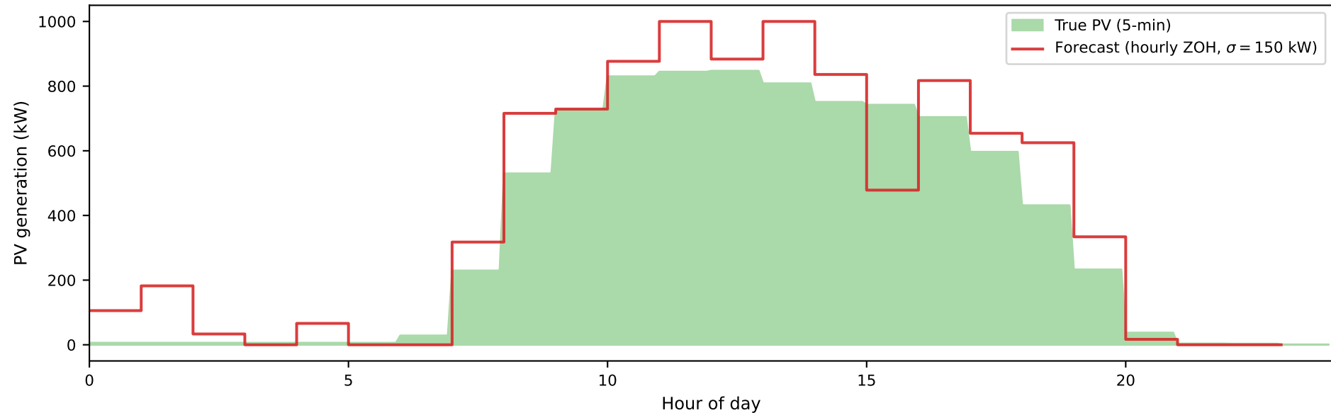
PV: True (5-min) vs Hourly Forecast — Day 1 (2024-07-08)
