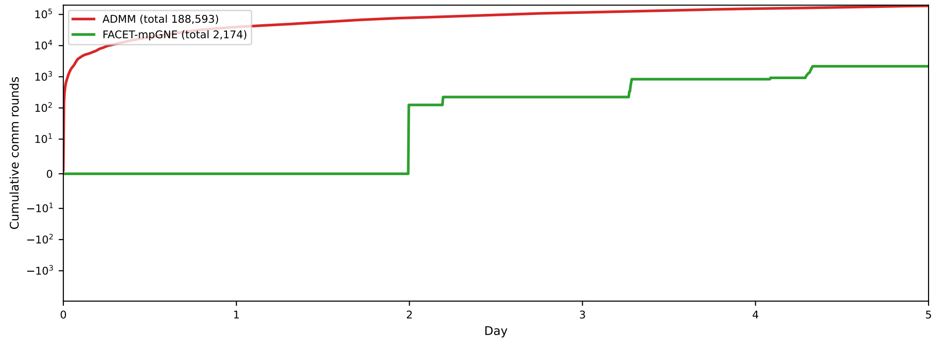
Cumulative comm rounds — 87× reduction with FACET
