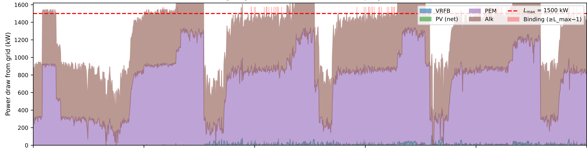
PCC coupling constraint active: 76/1440 steps (5.3%), Days 3-5 only
