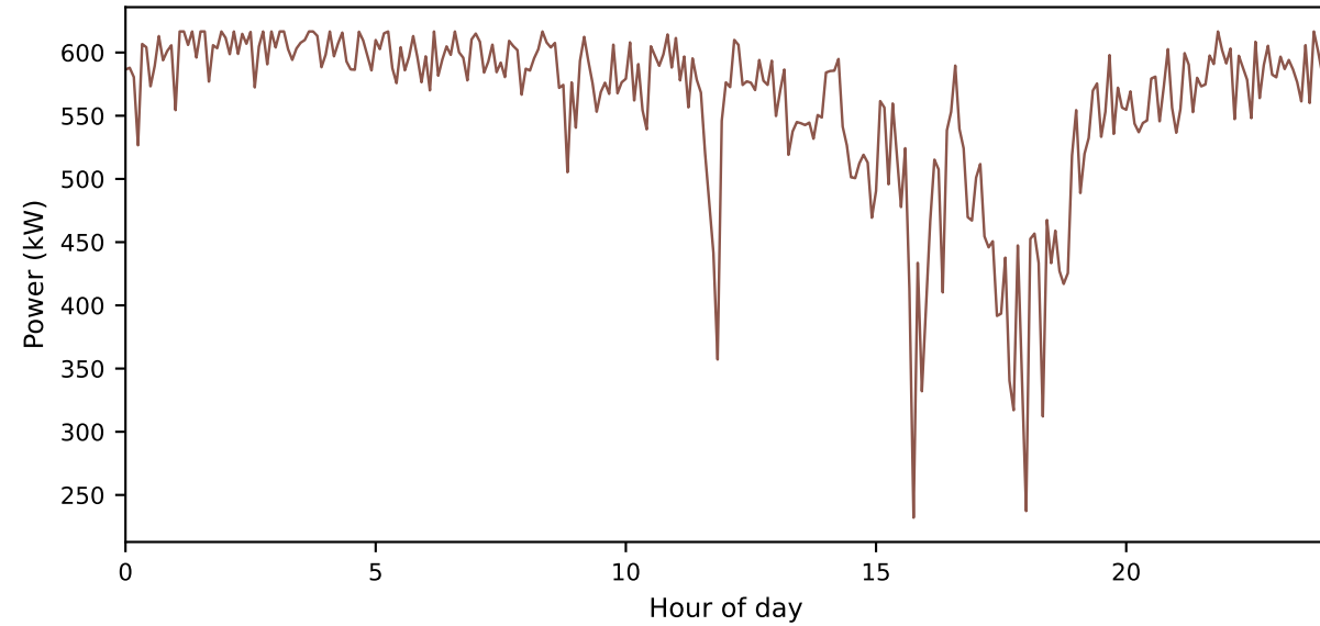
Alkaline — Day 1 (std=65.8 kW)
