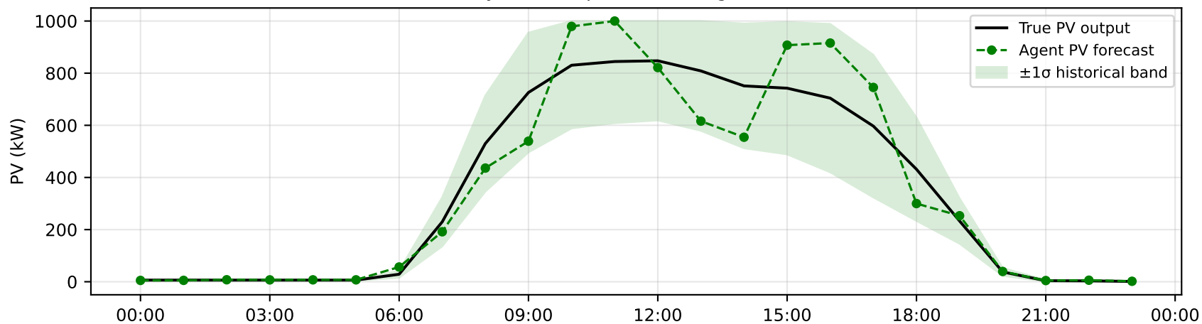
(b) Day 1 PV Output: True vs Agent Forecast
