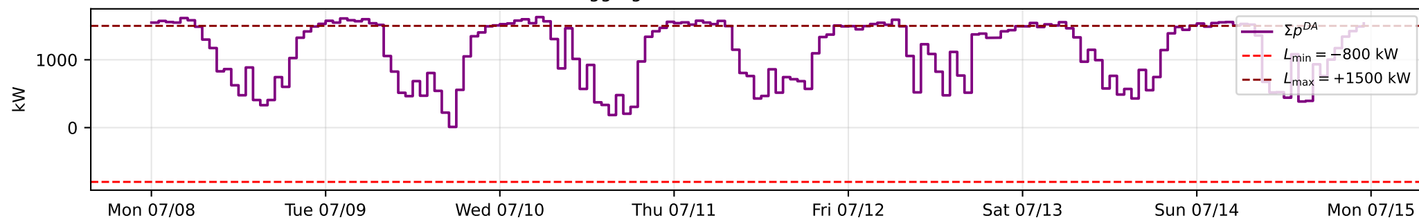
Aggregate DA Schedule vs PCC Bounds
