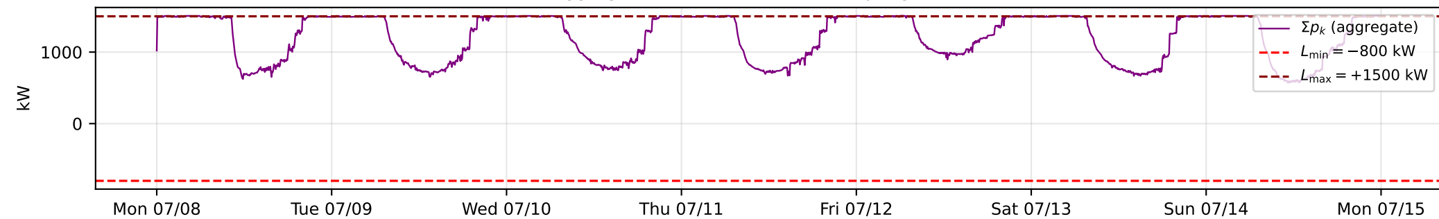
Aggregate RTM Power vs PCC Coupling Bounds
