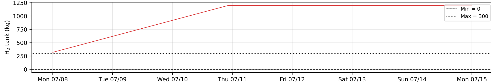
Agent 4: Alk Elz — State trajectory
