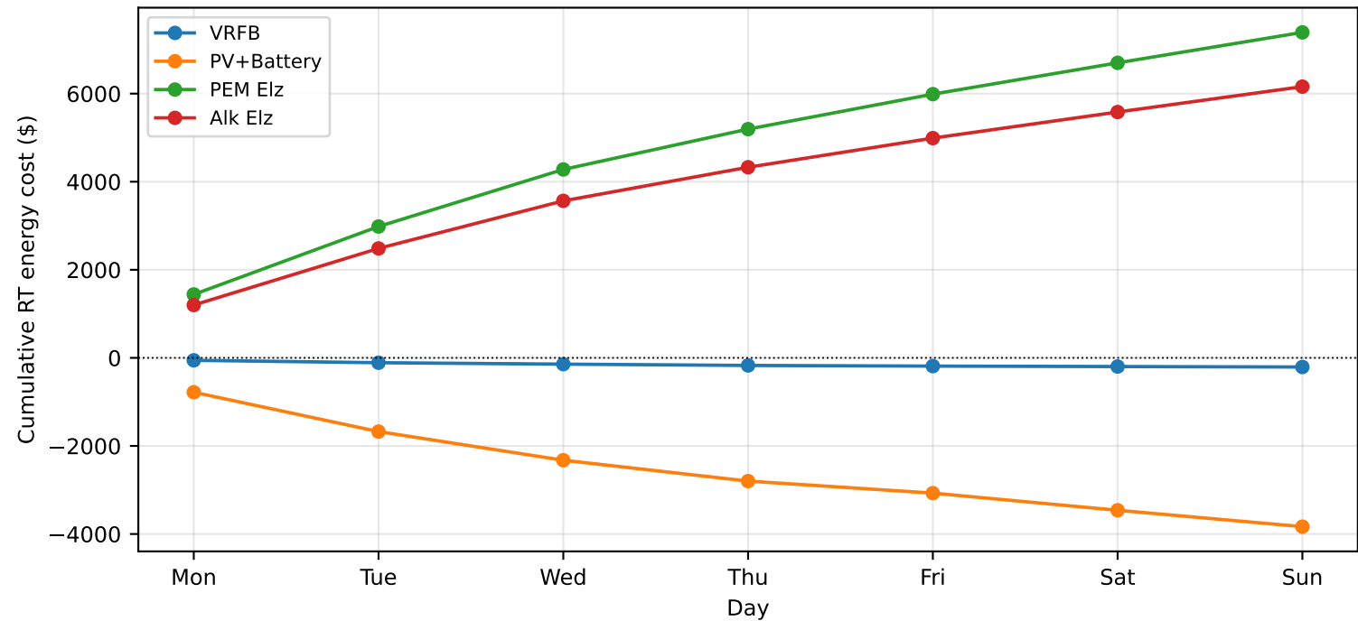
Cumulative RT Energy Cost per Agent Over 7-day PJM Simulation
