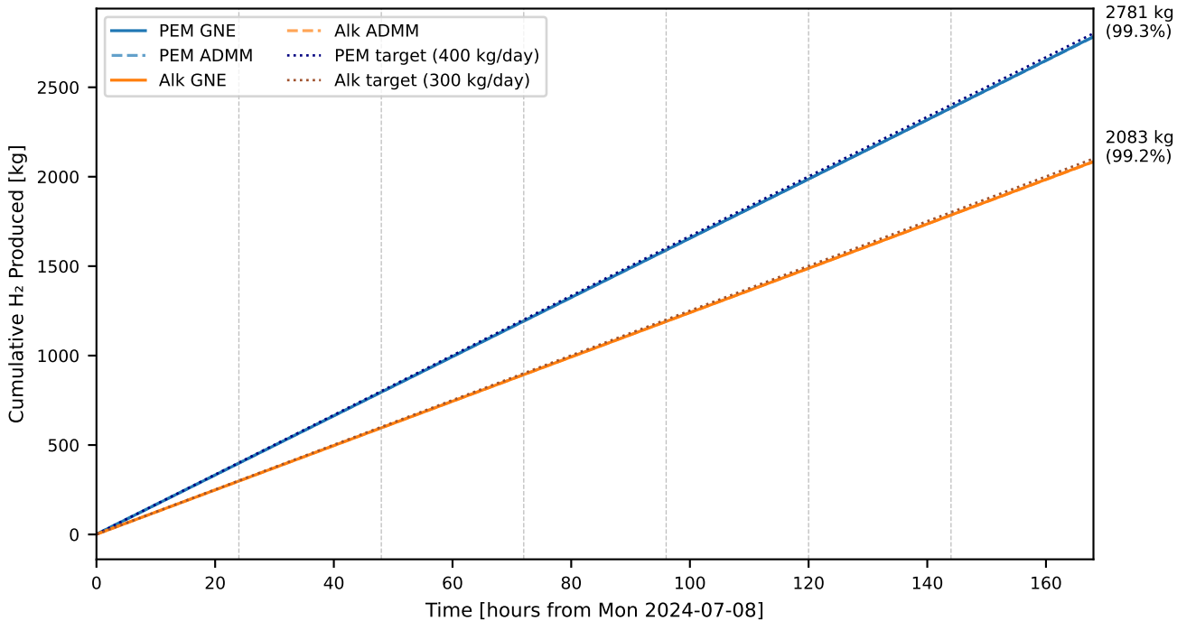
Cumulative H 2 Production vs. Take-or-Pay Target
