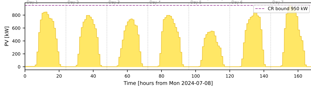
(c) 5-min PV Generation (1 MW capacity)
