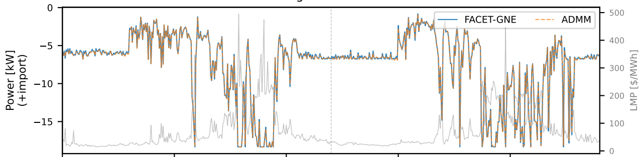
Agent 1: PV+Batt
