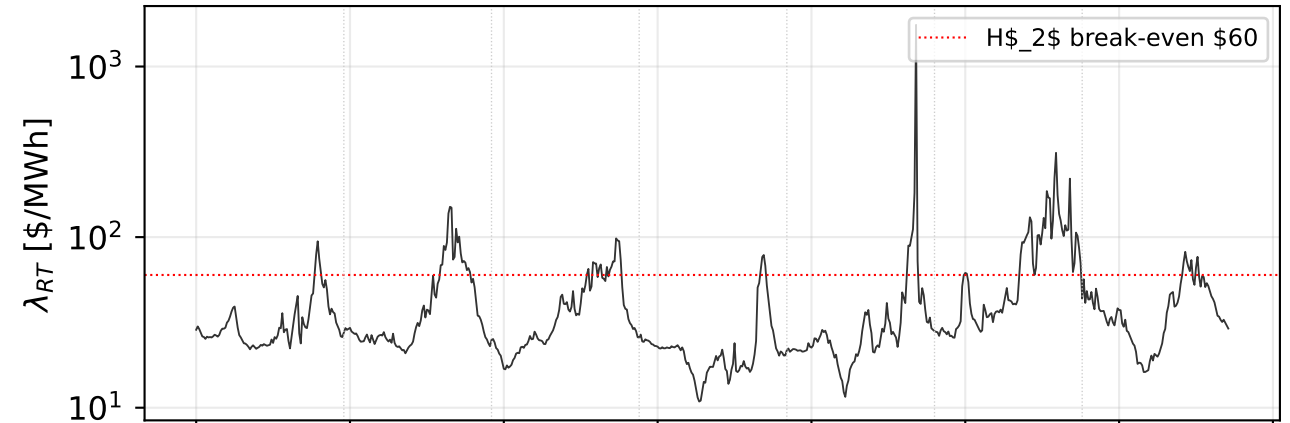
July 7-13: RT price
