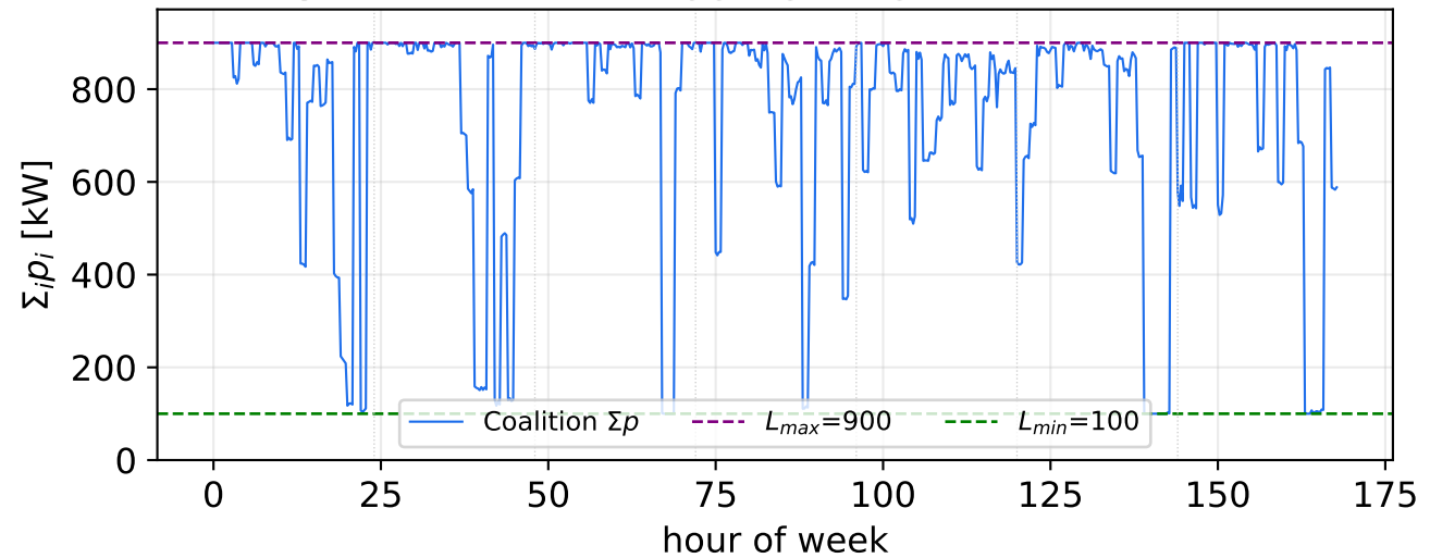
July 7-13: coalition aggregate grid import (FACET)
