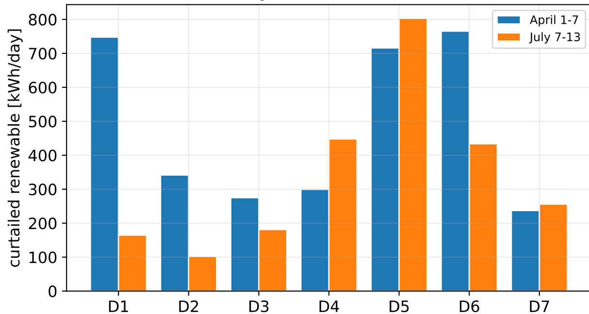
Daily fleet curtailment
