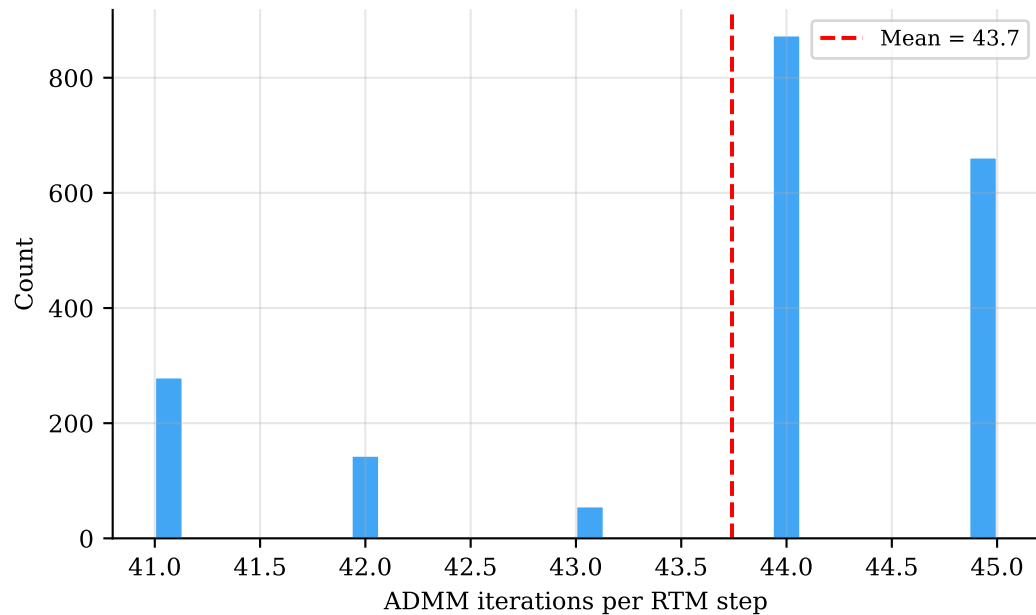
Iteration Histogram (2016 steps)
