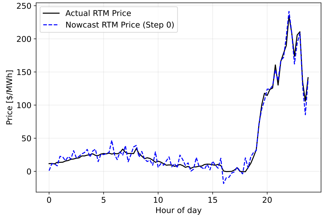
RTM Prices on 2025-04-06
