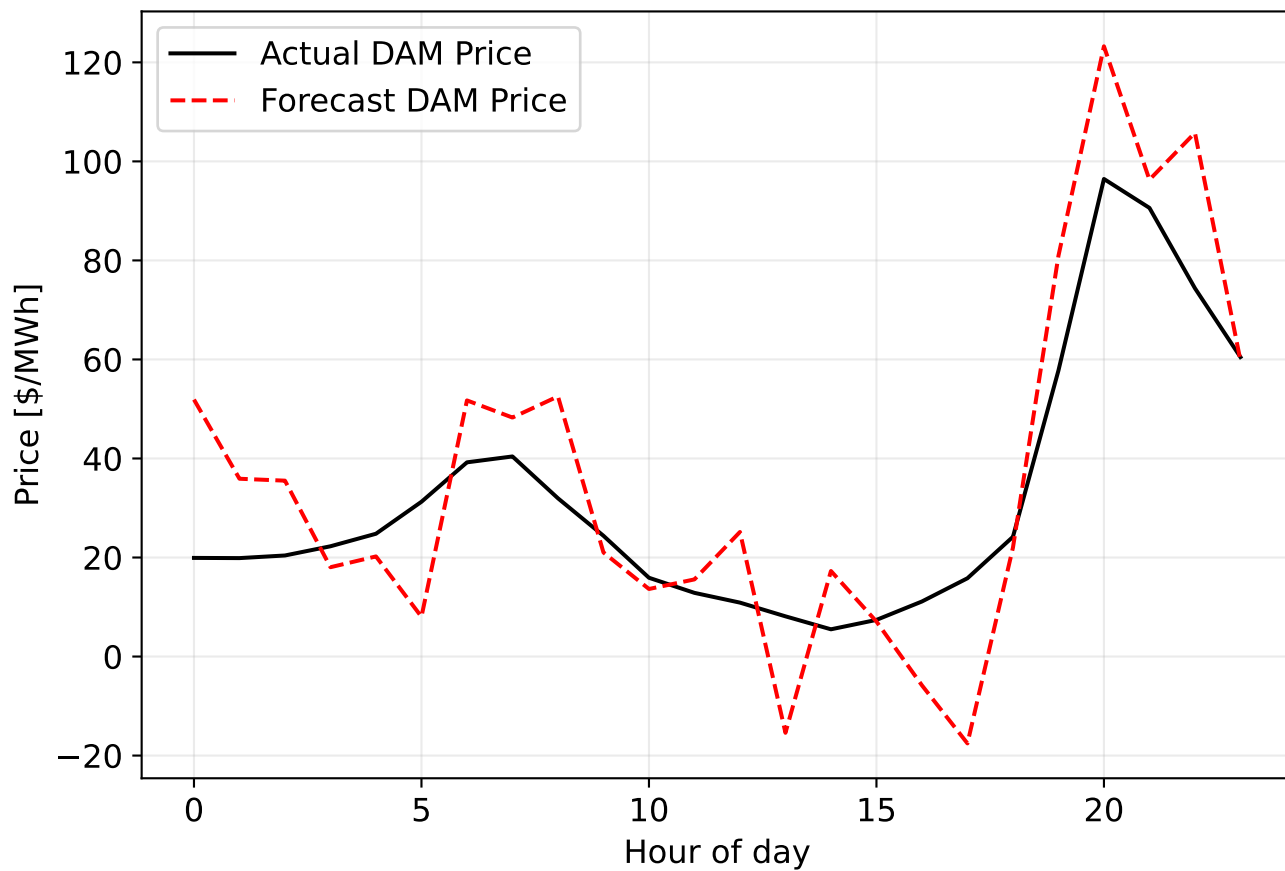
DAM Prices on 2025-04-06
