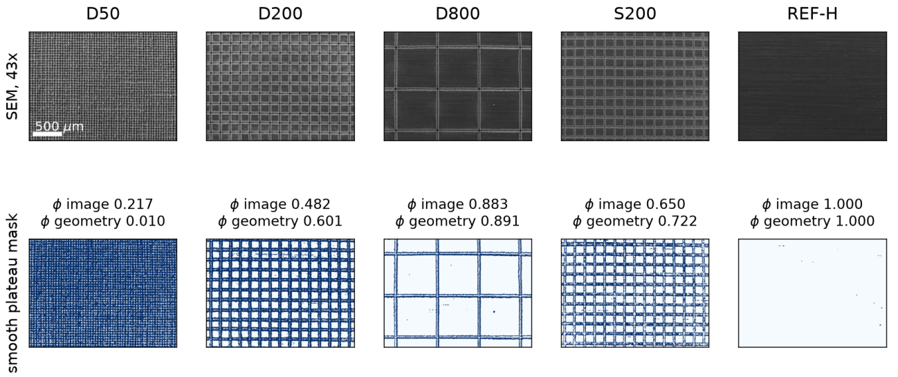
Figure 10. SEM image reader. Top: 43\times SEM images of four textured surfaces and the smooth REF-H plate (annotation bar removed; scale bar 500 \mu\text{m} ). Bottom: plateau mask (white = smooth plateau, blue = rough laser track) from the local-roughness map and the Otsu threshold fitted on textured images, with the resulting \phi and the \phi from nominal geometry, Eq. (3). The reader recovers \phi = 1.000 on REF-H, which it never saw in training.
