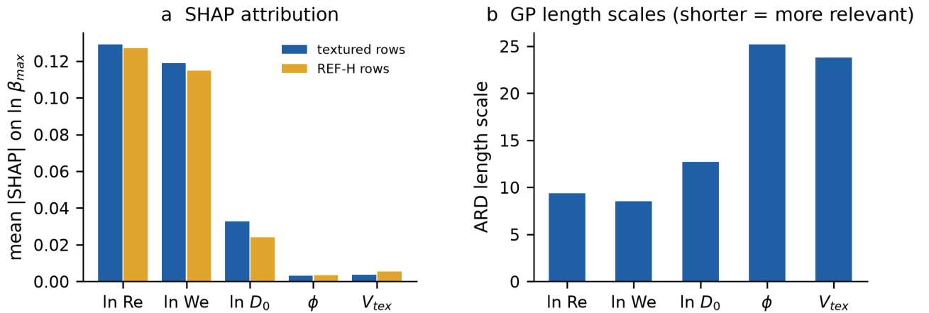
Figure 6. Input relevance for the final GP. (a) Mean absolute SHAP value [15] of each input on the predicted ln \beta_{max} (KernelExplainer, 20 k-means background points; 250 textured impacts and all 125 REF-H impacts). (b) Fitted ARD length scales of the Matérn kernel on standardised inputs; a shorter length scale means the output varies faster with that input. Both views rank ln Re and ln We first, ln D_0 third, and the texture descriptors last.
