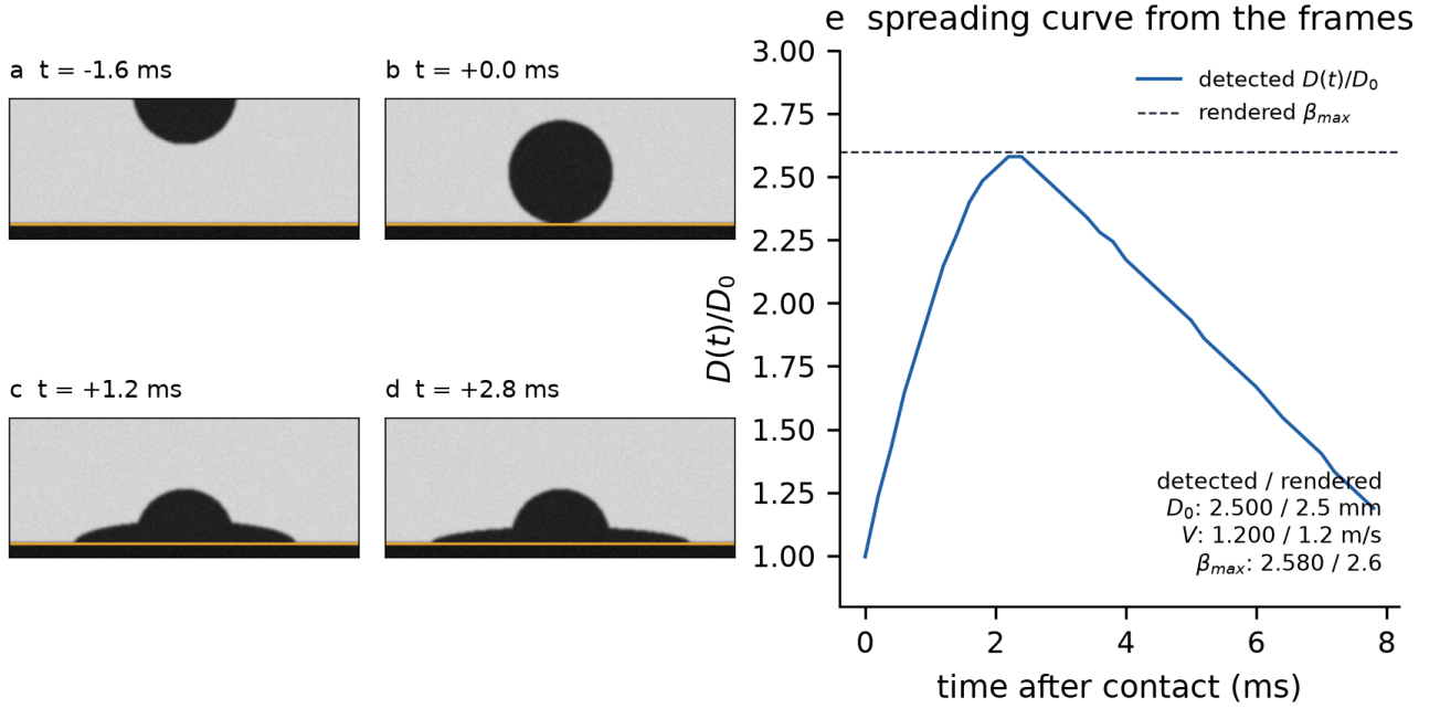
Figure 11. Video measurement on a synthetic test clip (true D_0 = 2.5 mm, V = 1.2 m/s, \beta_{\max} = 2.6 , 5,000 fps, 0.03 mm/px). (a–d) Frames before contact, at contact and during spreading; the orange line is the automatically detected substrate. (e) Spreading diameter D(t)/D_0 detected from every frame, with the rendered \beta_{\max} (dashed). The inset text compares detected and rendered values. This verifies the software, not its accuracy on real footage.
