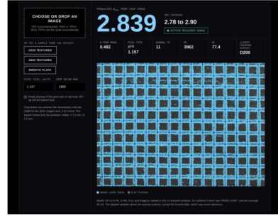
b Prediction from an SEM image
