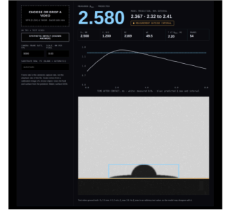
c Measurement from video
