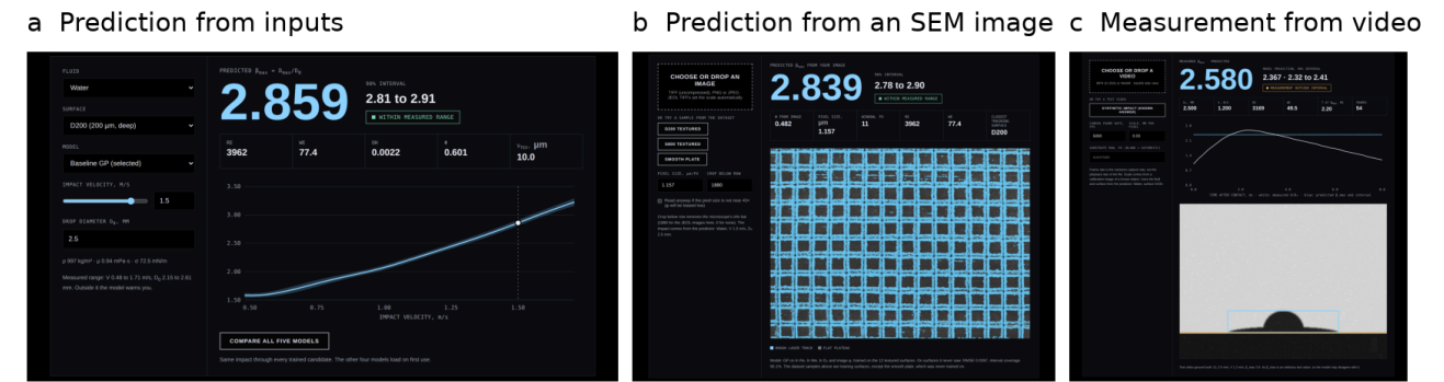
Figure 12. The interface running the same GP in the browser. (a) Prediction from fluid, surface, D_0 and V , with the calibrated 90% interval, the dimensionless groups and the velocity response curve. (b) Prediction from an uploaded 43× SEM image (D200 shown): rough laser tracks are highlighted, \varphi is read from the image and the image-only GP predicts \beta_{\max} . (c) Automatic measurement from an uploaded side-view video (synthetic test clip). The arbitrary test \beta_{\max} of 2.6 lies outside the model's interval for that impact on D200, and the interface reports the disagreement instead of hiding it.
