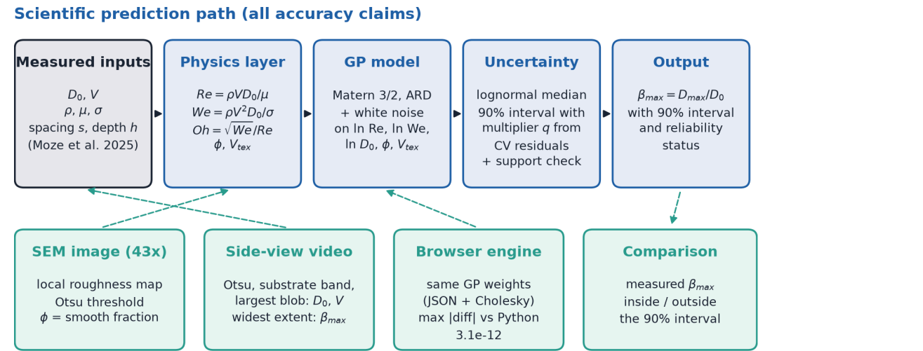
Figure 1. System architecture. Top: the scientific prediction path, which carries every accuracy claim in this paper. Bottom: the measurement and interface path. The SEM reader supplies \phi , the video pipeline supplies D_0 and V (and a measured \beta_{\max} for comparison), and the browser engine evaluates the same GP weights. Dashed arrows show where each front end connects to the prediction path.
