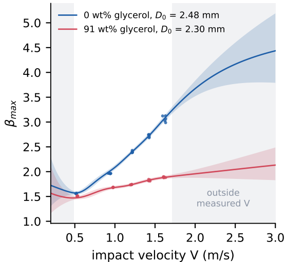
b GP median and 90% interval on D200
