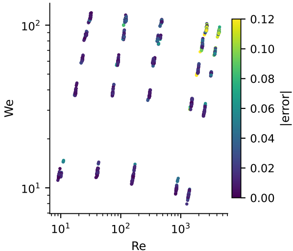
a |LOSO error| of the GP
